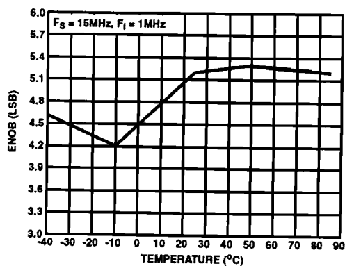
FIGURE 13. ENOB vs TEMPERATURE
