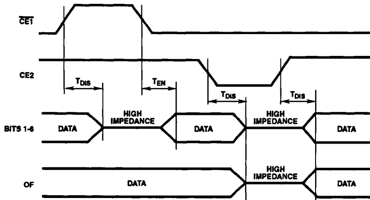
FIGURE 2. OUTPUT ENABLE
