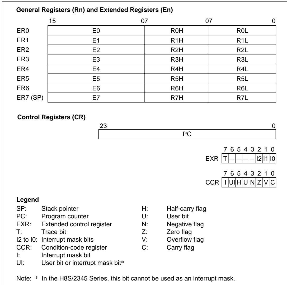
Figure 2.7 CPU Registers
