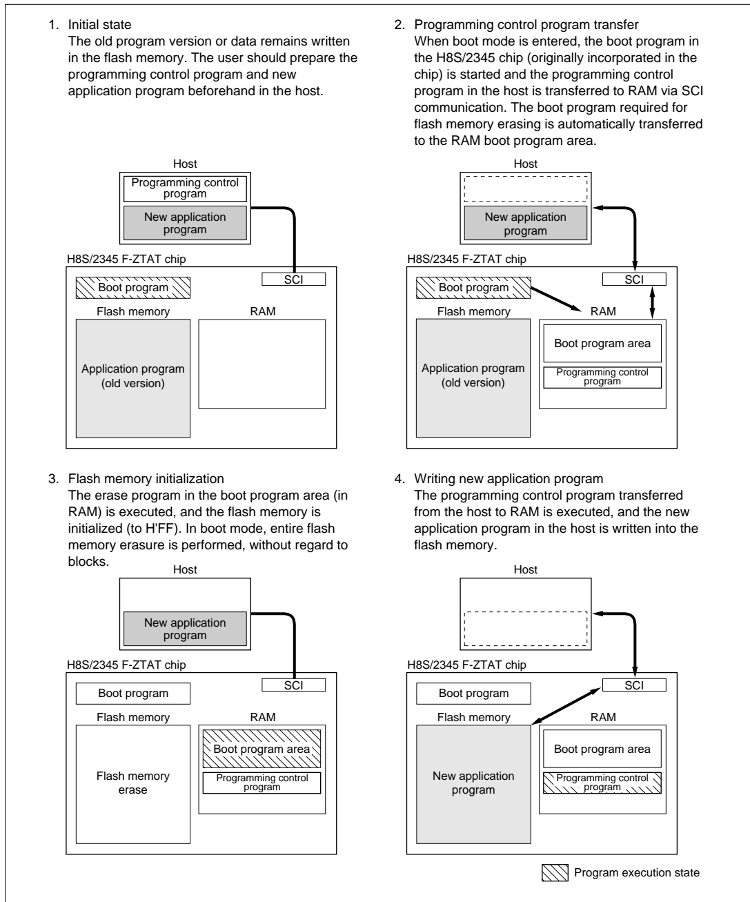
Figure 17.9 Boot Mode
