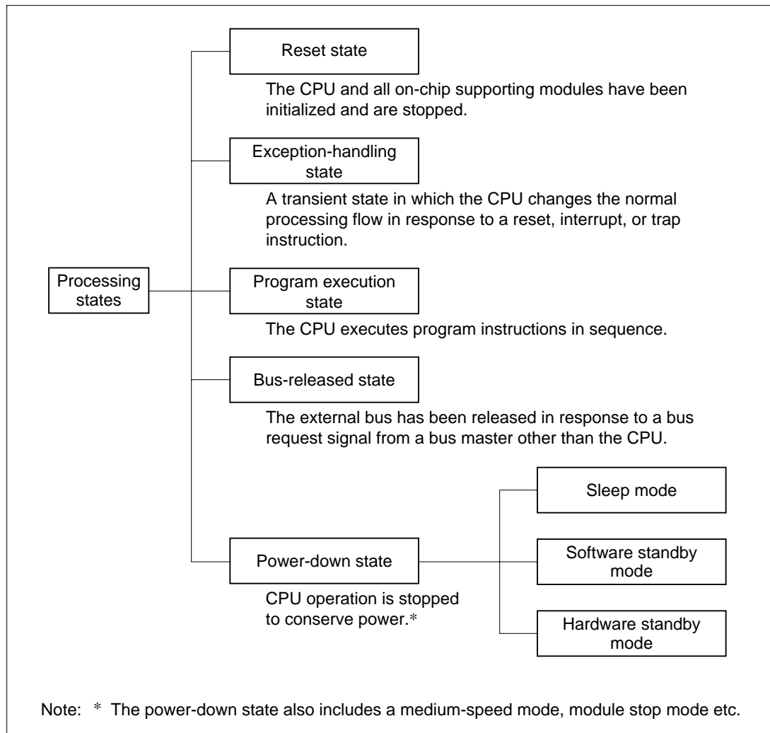
Figure 2.14 Processing States
