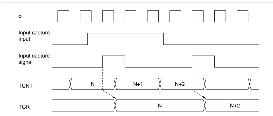
Figure 9.37 Input Capture Input Signal Timing
