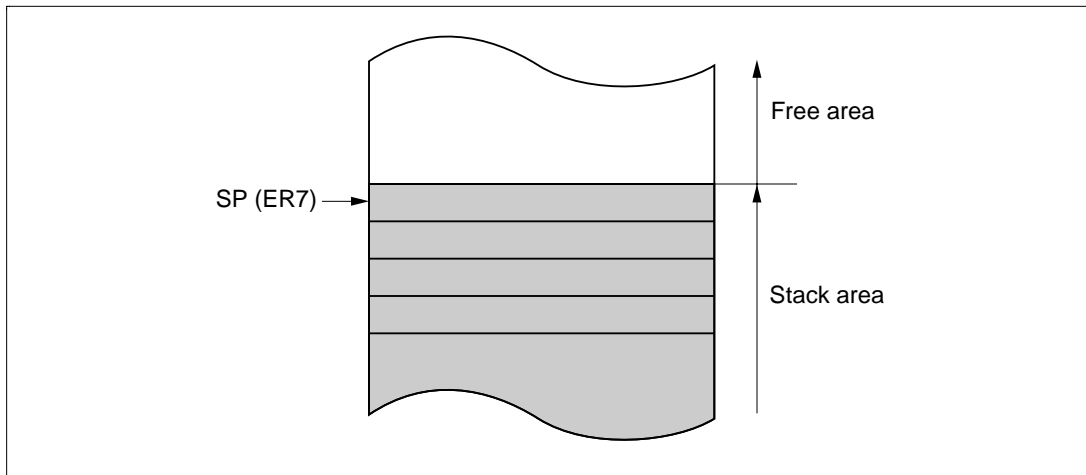
Figure 2.9 Stack
