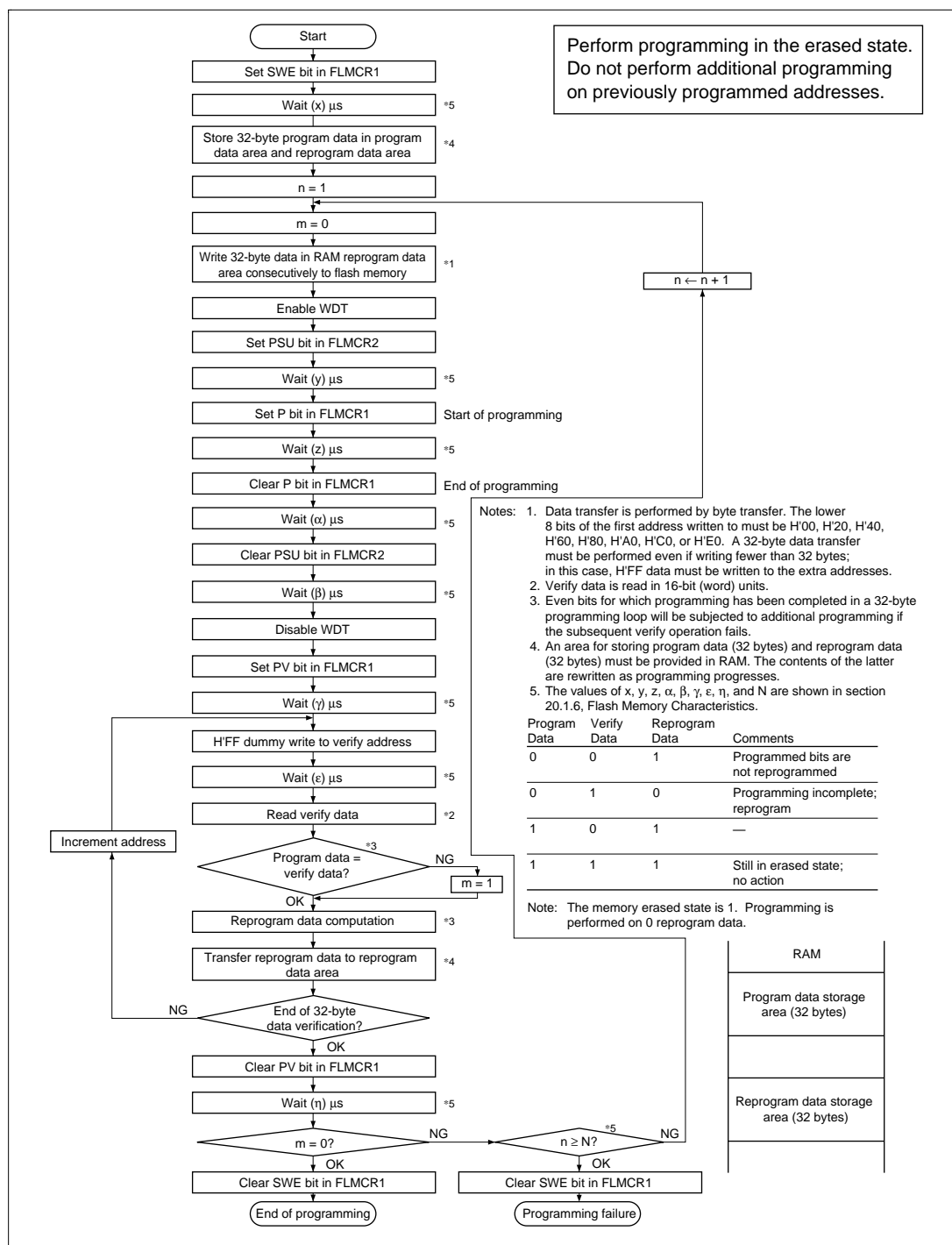
Figure 17.21 Program/Program-Verify Flowchart
