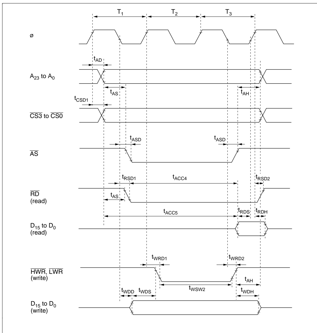
Figure 20.12 Basic Bus Timing (Three-State Access)
