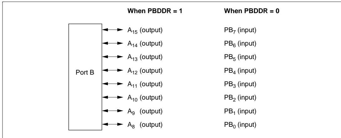
Figure 8.11 Port B Pin Functions (Modes 2 and 6) *
