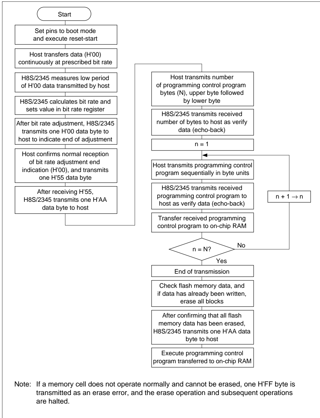
Figure 17.16 Boot Mode Execution Procedure
