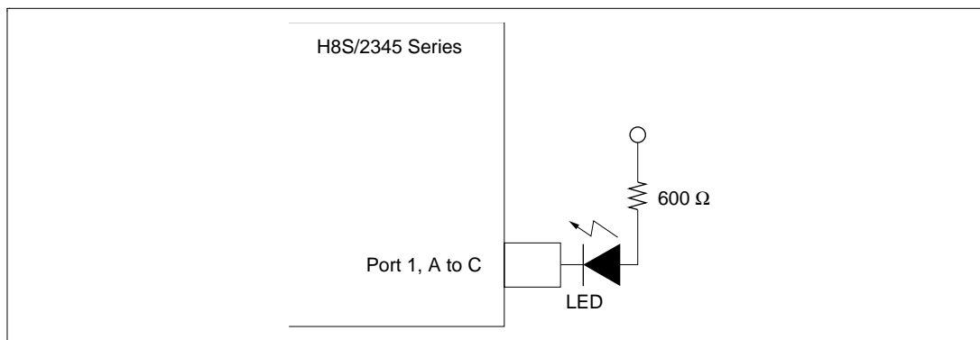
Figure 20.2 LED Drive Circuit (Example)
