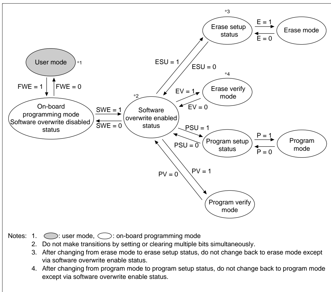
Figure 17.20 Mode Transitions Using Settings of Bits in FLPCR1 and FLPCR2
