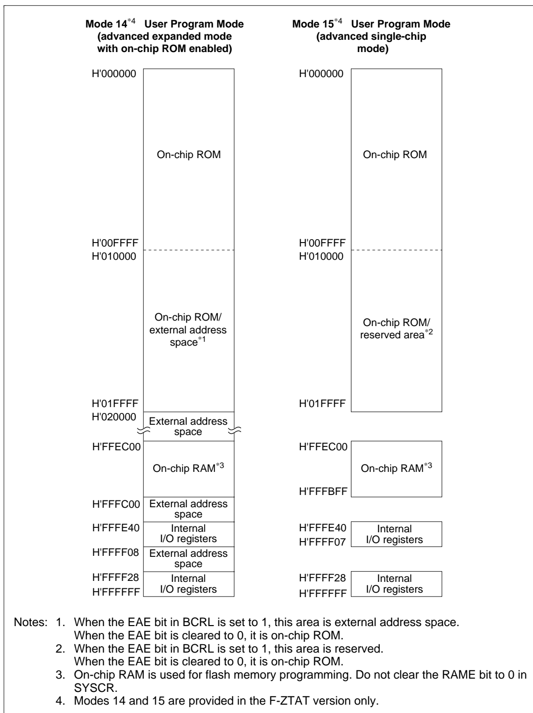
Figure 3.1 Memory Map in Each Operating Mode in the H8S/2345 (cont)
