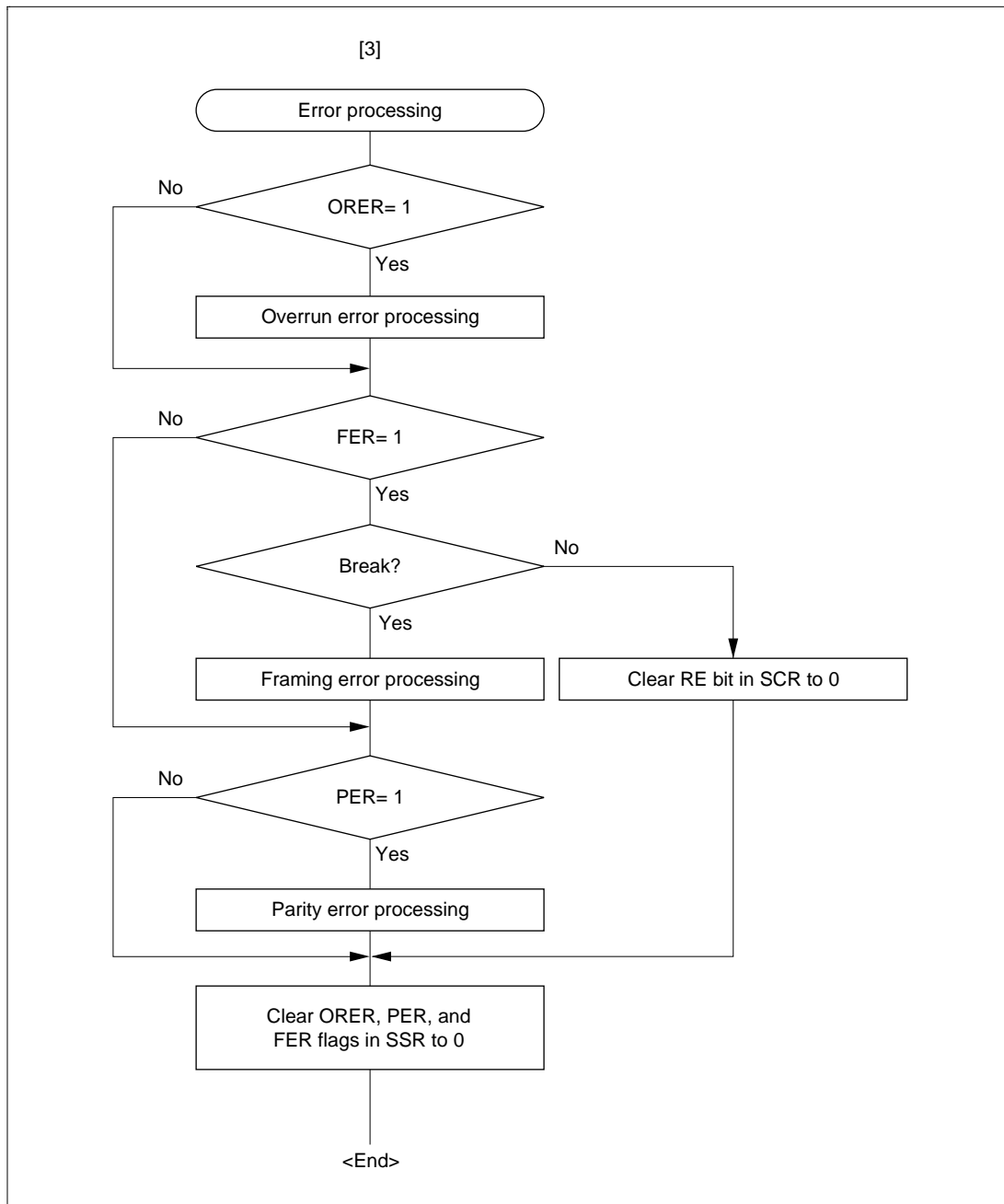
Figure 12.7 Sample Serial Reception Data Flowchart (cont)
