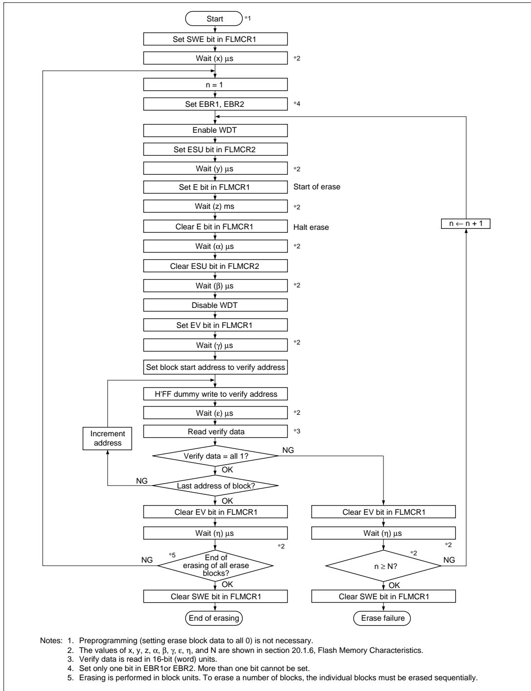
Figure 17.22 Erase/Erase-Verify Flowchart (Single-Block Erase)
