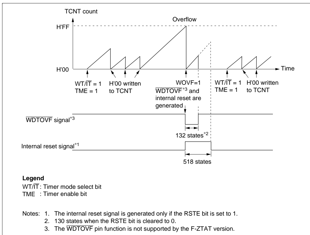
Figure 11.4 Watchdog Timer Operation
