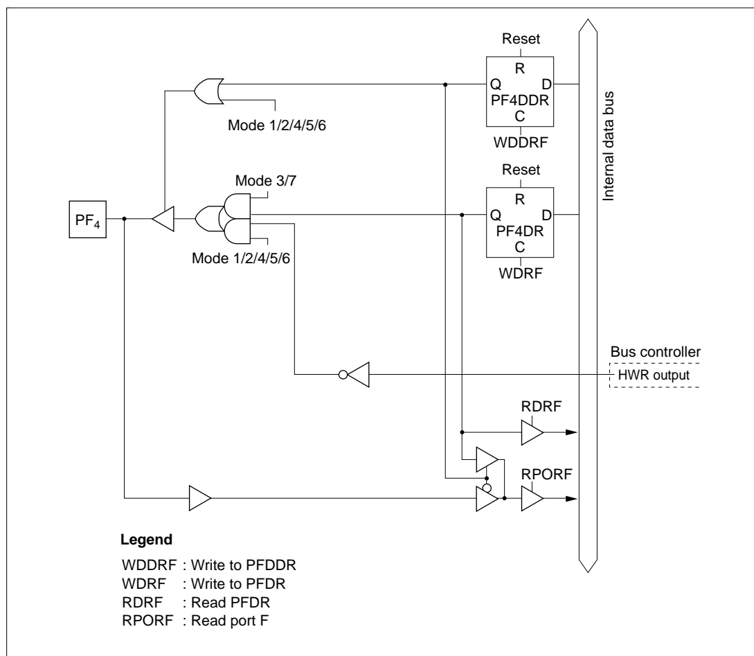
Figure C.10 (e) Port F Block Diagram (Pin PF 4 )
