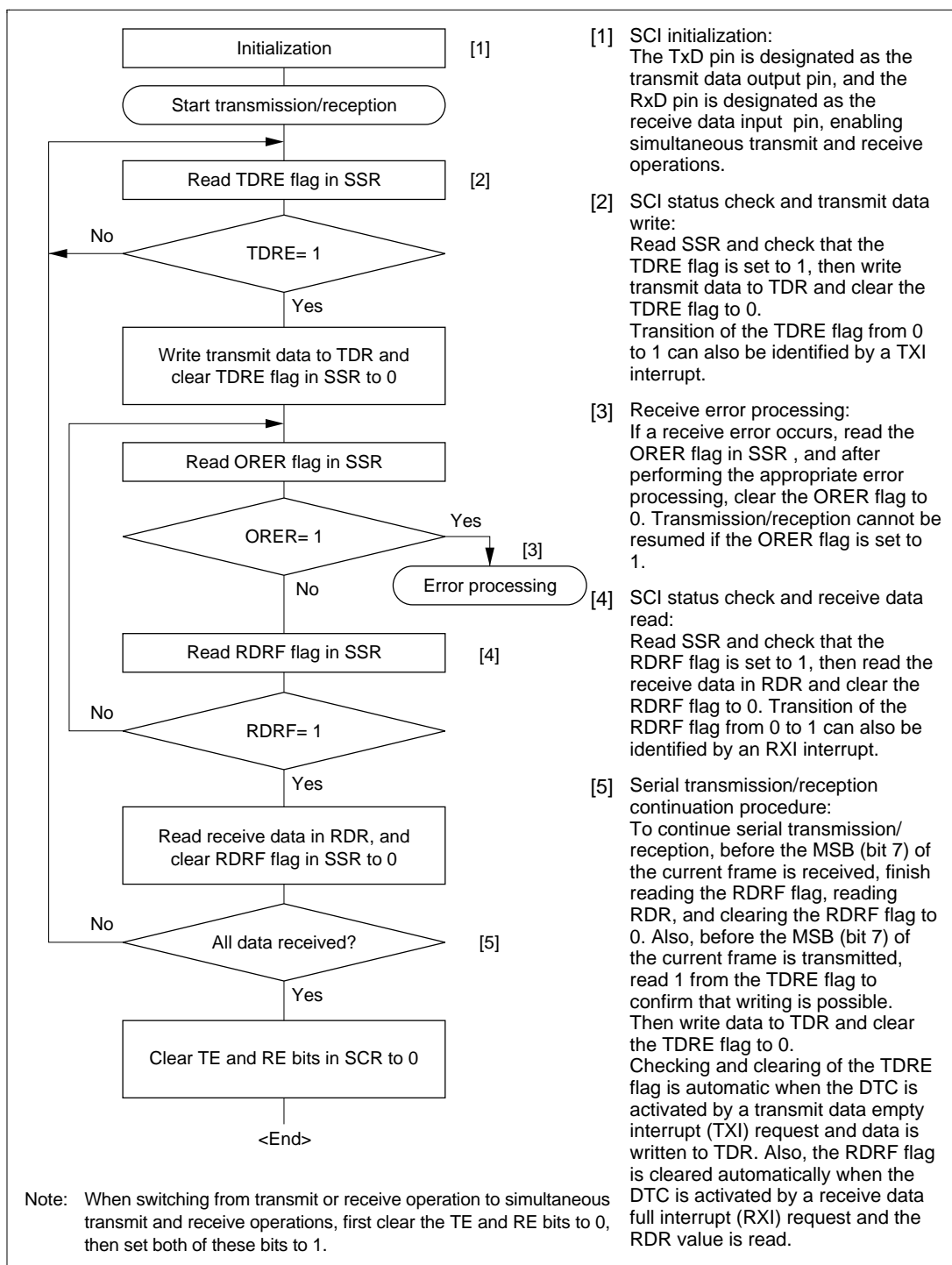
Figure 12.20 Sample Flowchart of Simultaneous Serial Transmit and Receive Operations
