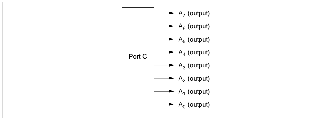
Figure 8.14 Port C Pin Functions (Modes 1, 4, and 5)*
