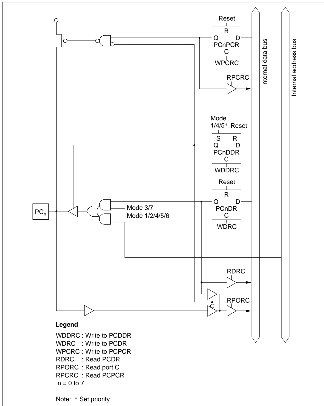
Figure C.7 Port C Block Diagram (Pin PC_n )
