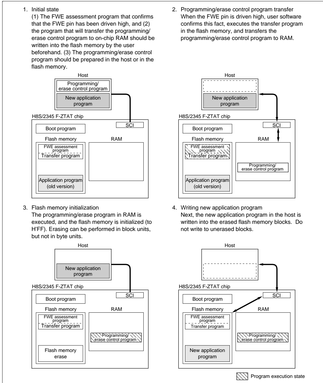
Figure 17.10 User Program Mode (Example)
