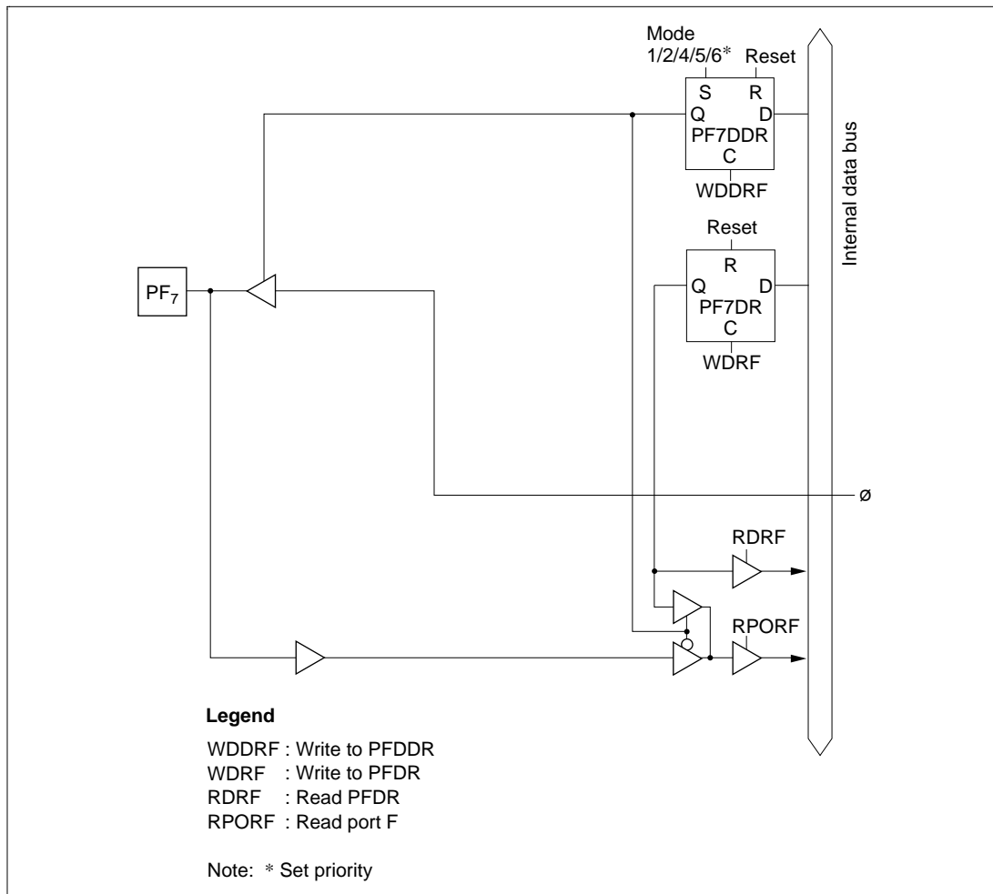
Figure C.10 (h) Port F Block Diagram (Pin PF 7 )
