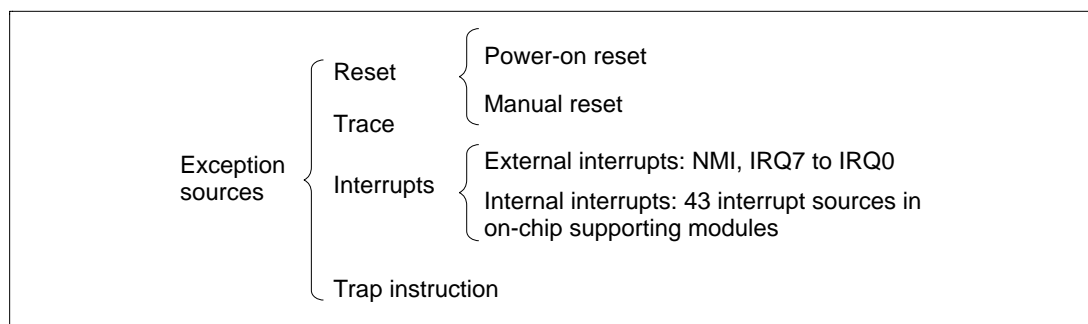
Figure 4.1 Exception Sources
