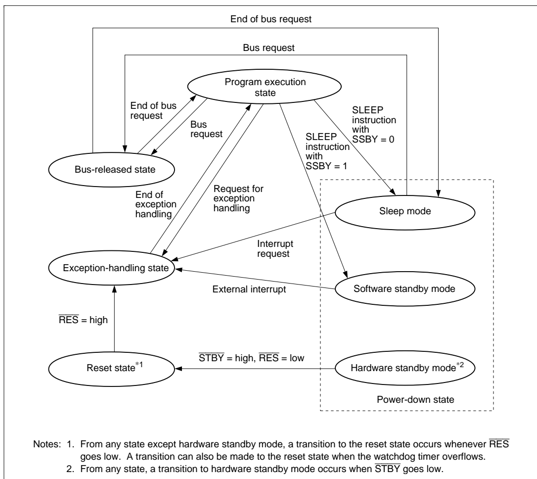
Figure 2.15 State Transitions
