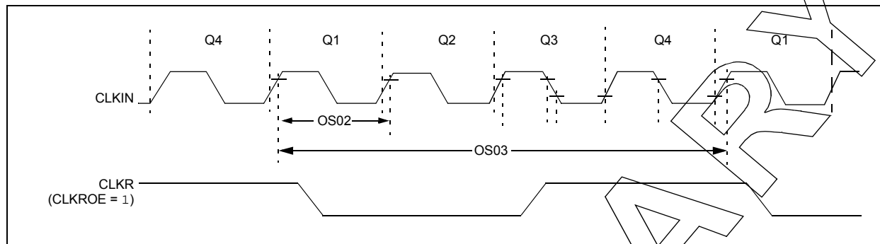
FIGURE 24-5: CLOCK TIMING
