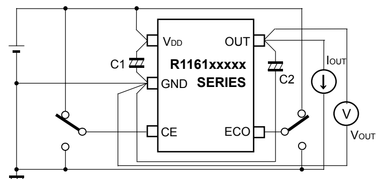
Fig.4 Output Voltage vs. Temperature Test Circuit
