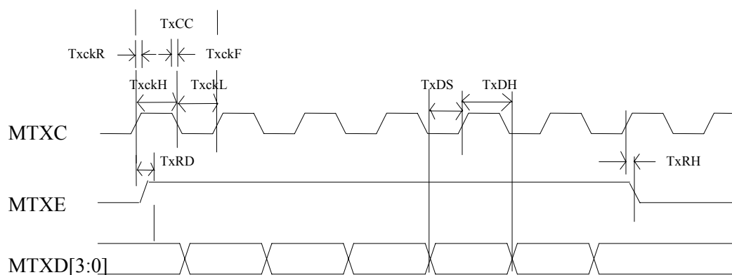
MI I Port – Transmit
