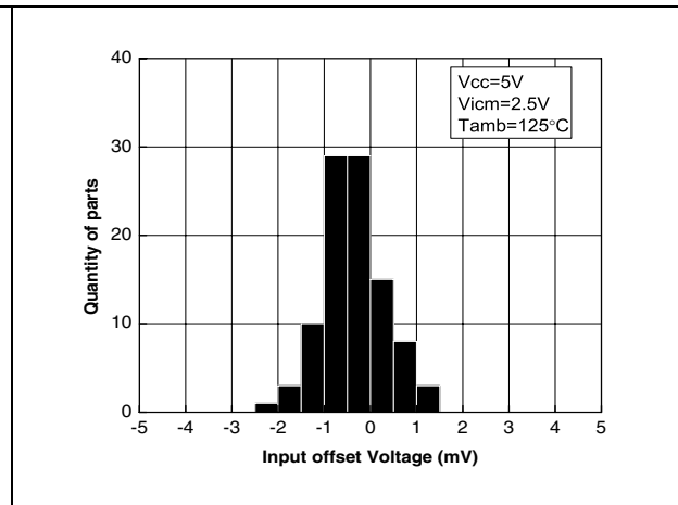
Figure 2. Input offset voltage distribution at T = 125^{\circ}\text{C}
