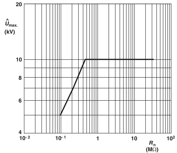
Maximum allowed peak pulse voltage in accordance with IEC 60065, 14.1.a); 50 discharges from a 1 nF capacitor charged to Umax-hat; 12 discharges/min (drift ΔR/R ≤ 2 %)
