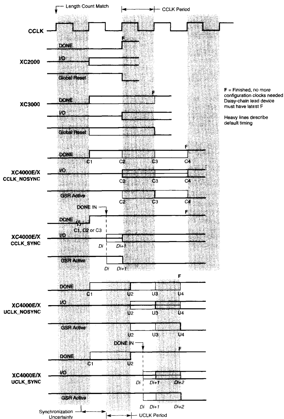
Figure 48: Start-up Timing
