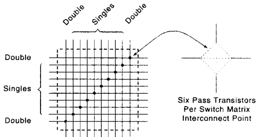
Figure 27: Programmable Switch Matrix (PSM)
