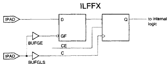
Figure 18: Examples Using XC4000X FCL
