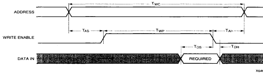
Figure 9: Level-Sensitive RAM Write Timing
