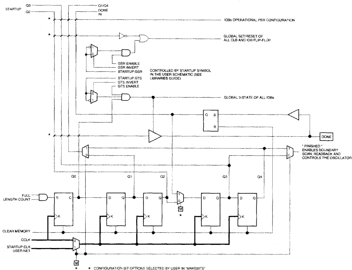
Figure 49: Start-up Logic
