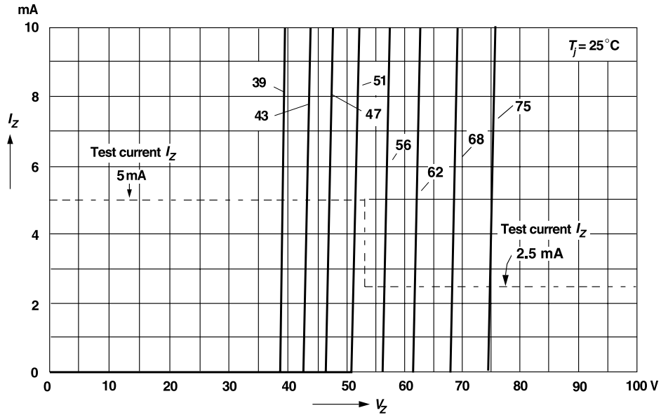
Figure 18. Breakdown Characteristics
