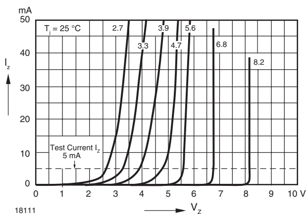
Figure 16. Breakdown Characteristics
