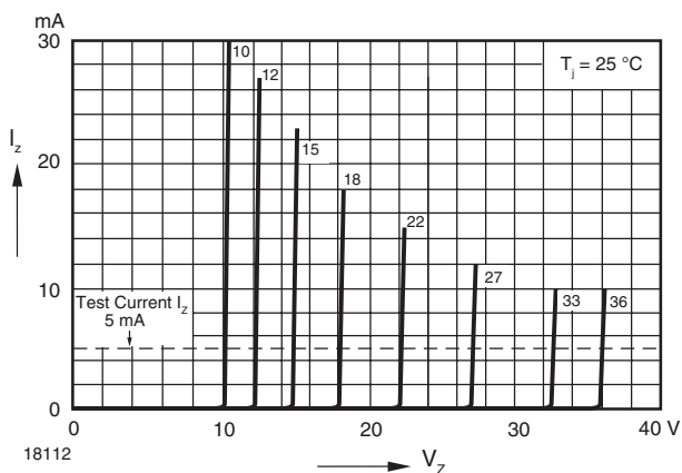
Figure 17. Breakdown Characteristics
