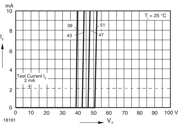
Figure 18. Breakdown Characteristics
