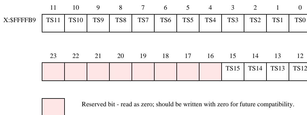
Figure 6-15 TSMA Register
