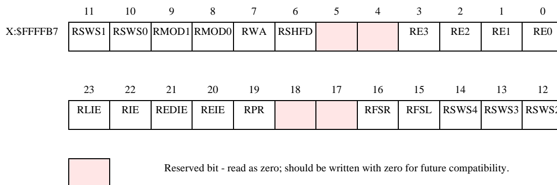
Figure 6-9 RCR Register
