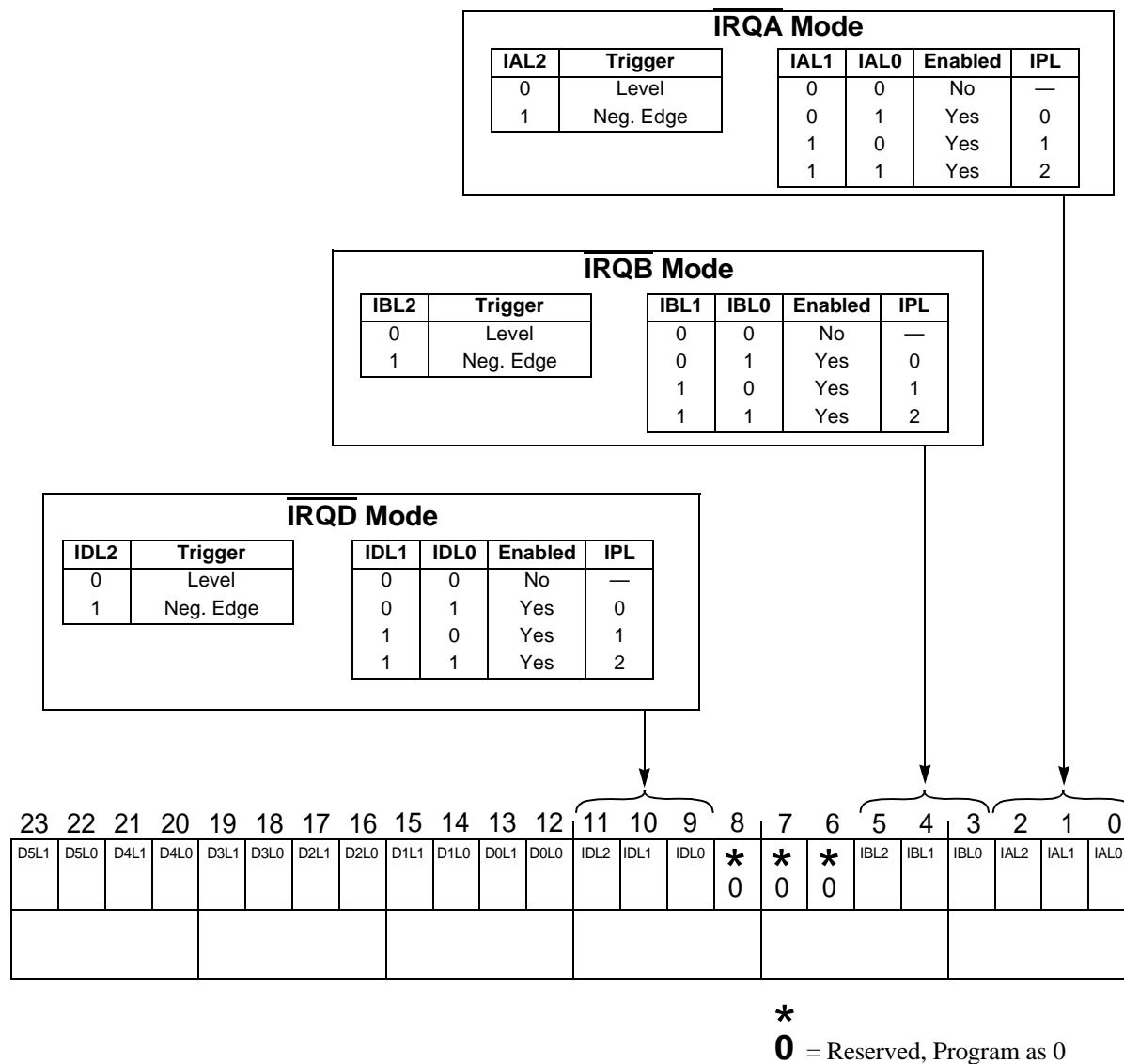
Figure C-3 Interrupt Priority Register-Core (IPR-C)
