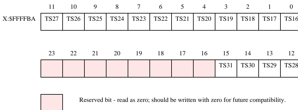
Figure 6-16 TSMB Register
