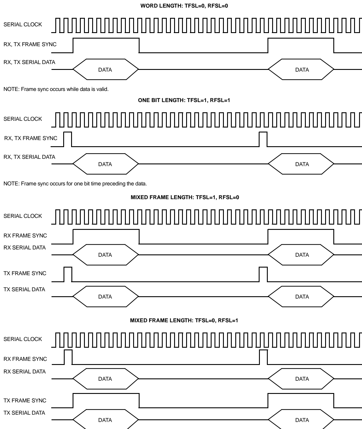
Figure 6-7 Frame Length Selection
