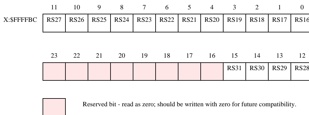
Figure 6-18 RSMB Register
