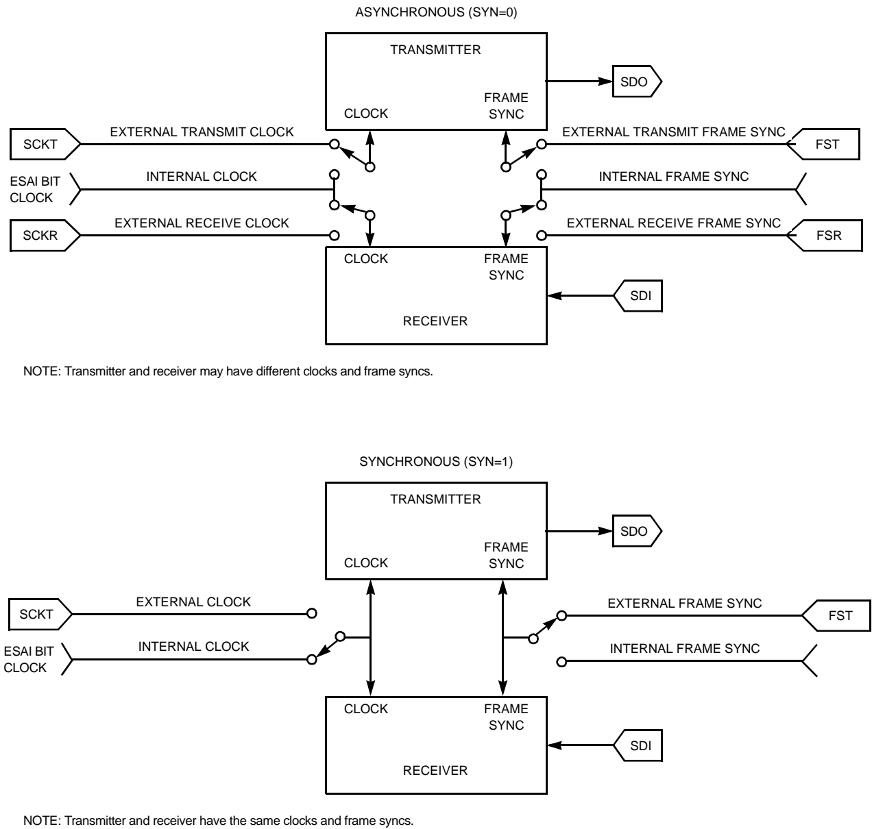
Figure 6-11 SAICR SYN Bit Operation
