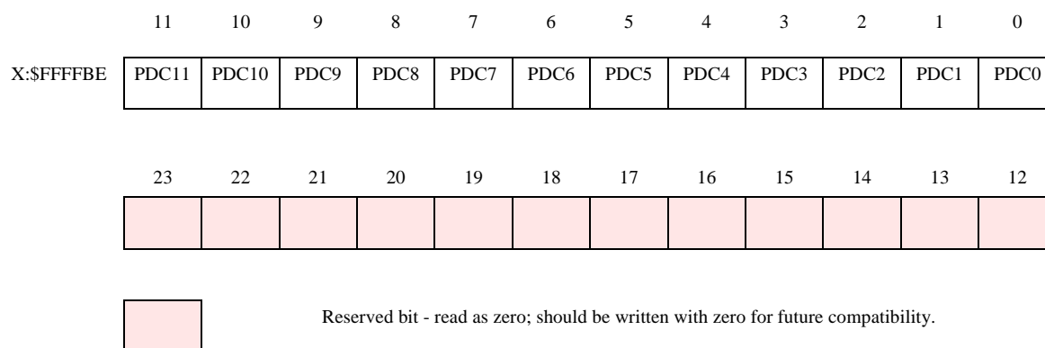
Figure 6-20 PRRC Register
