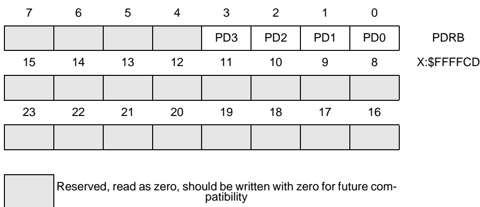
Figure 5-3 GPIO Port B Data Register (PDRB)
