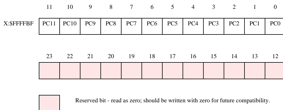
Figure 6-19 PCRC Register
