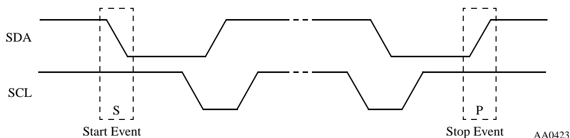
Figure 7-8 I 2 C Start and Stop Events
