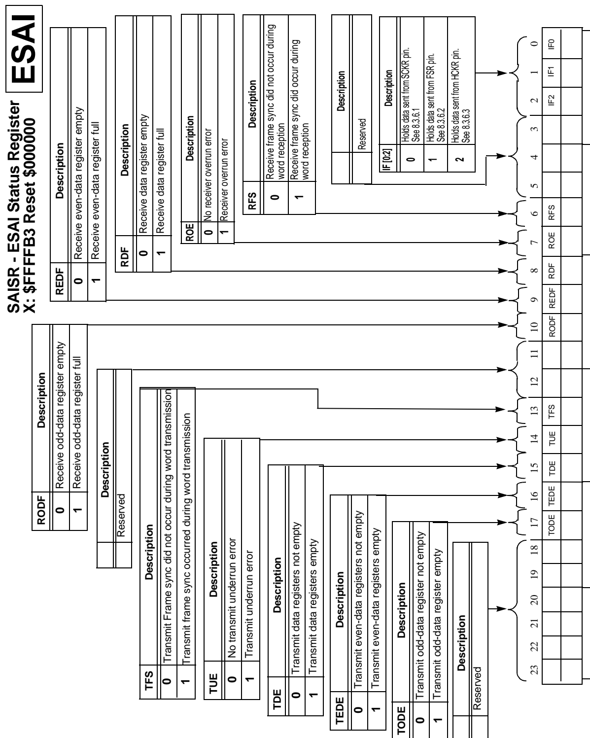
Figure C-14 ESAI Status Register (SAISR)
