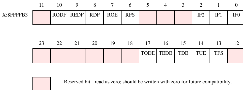
Figure 6-12 SAISR Register
