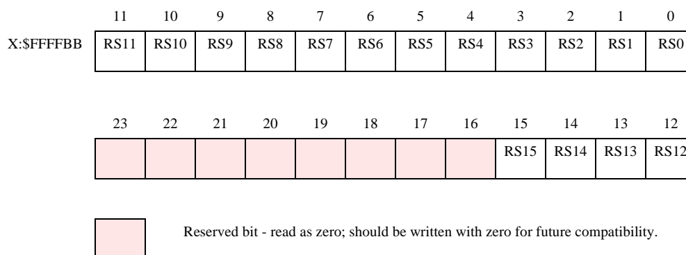
Figure 6-17 RSMA Register
