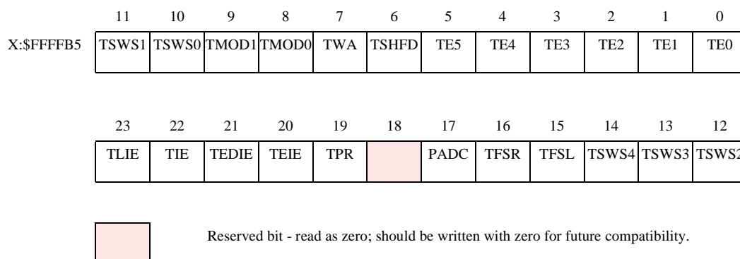
Figure 6-5 TCR Register
