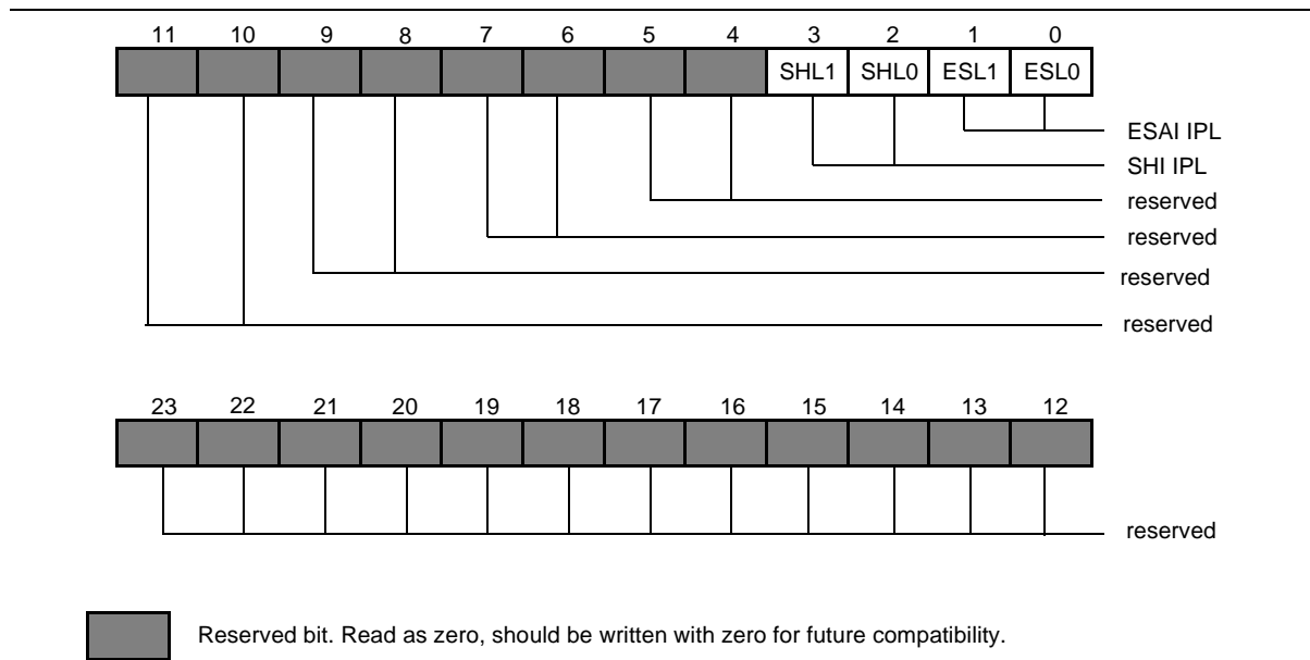
Figure 4-2 Interrupt Priority Register P
