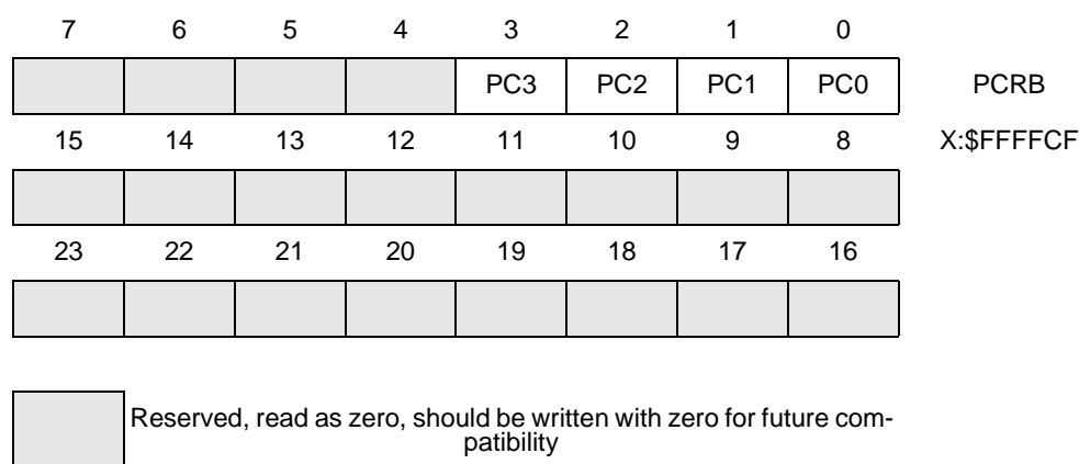
Figure 5-1 GPIO Port B Control Register (PCRB)
