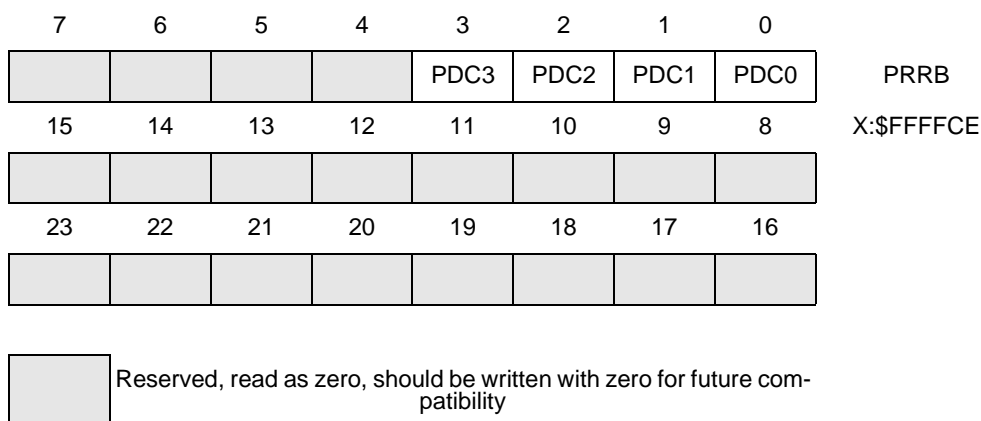
Figure 5-2 GPIO Port B Direction Register (PRRB)
