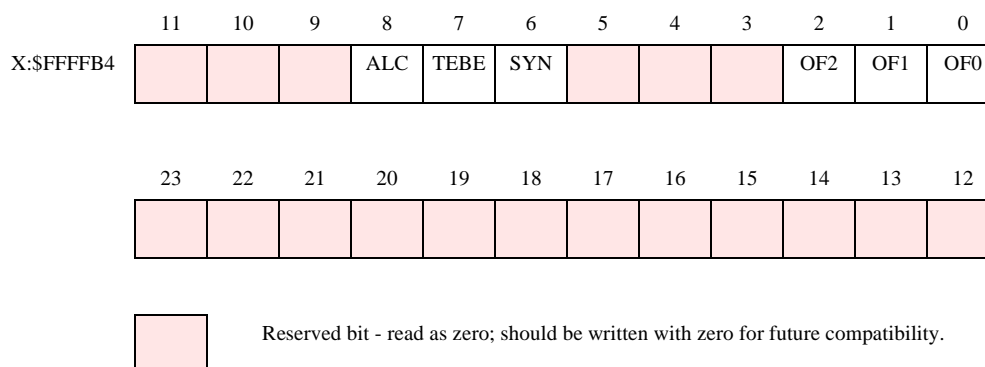
Figure 6-10 SAICR Register
