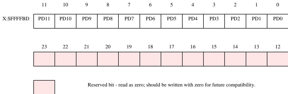
Figure 6-21 PDRC Register
