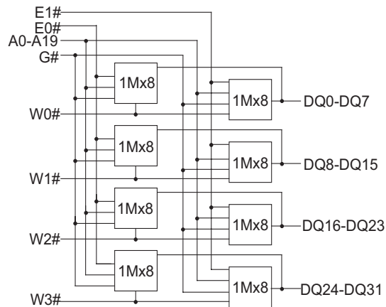
ED17F2331MC-BNC: 2x1Mx32 80 PIN
