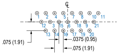
21 PIN
