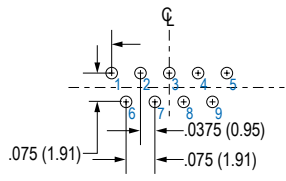
9 PIN
