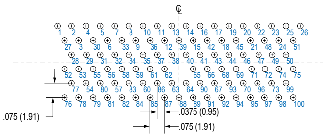
100 PIN
