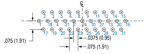
31 PIN
