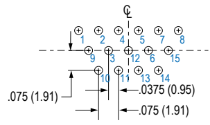
15 PIN
