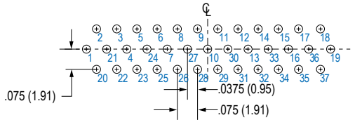
37 PIN
