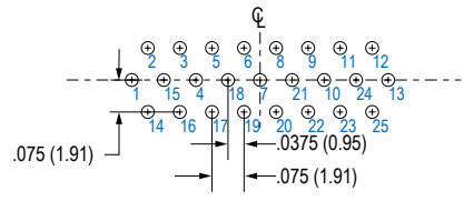
25 PIN
