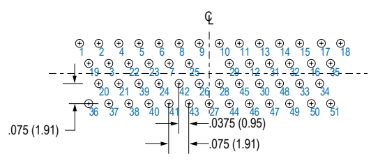
51 PIN
