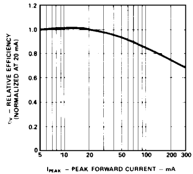
Figure 4. Relative Efficiency vs. Peak Forward Current.
