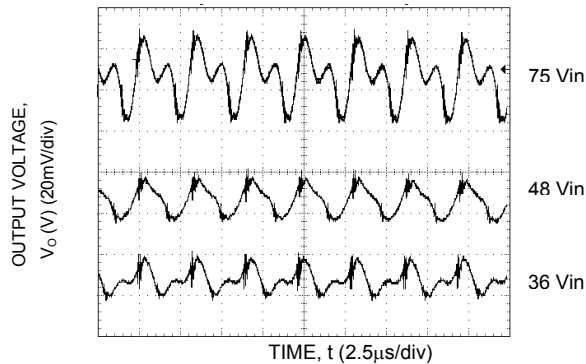
Figure 21. Typical Output Ripple and Noise at Room Temperature and I_o = I_{o, max} .
