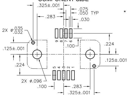
PLUG PC BOARD LAYOUT COMPONENT SIDE
