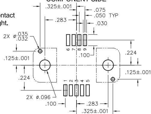
RECEPTACLE PC BOARD LAYOUT COMPONENT SIDE
