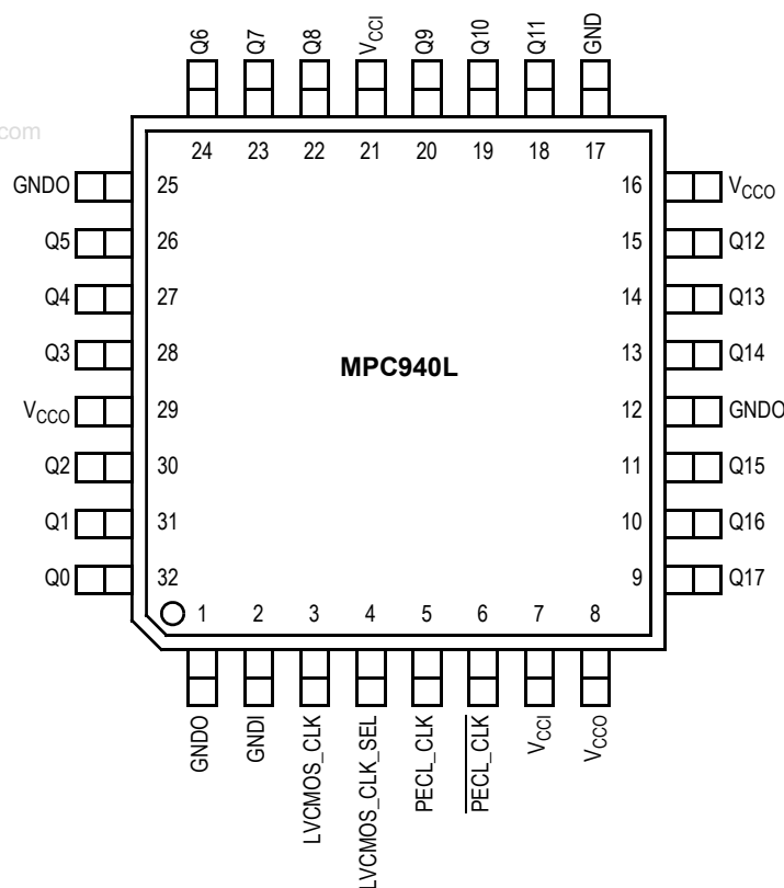
Pinout: 32-Lead LQFP (Top View)
