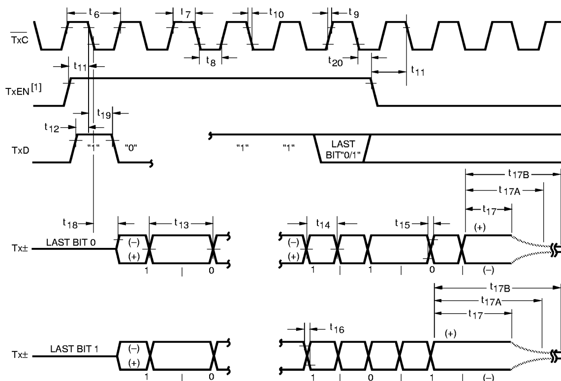
Figure 7. Transmit Timing
