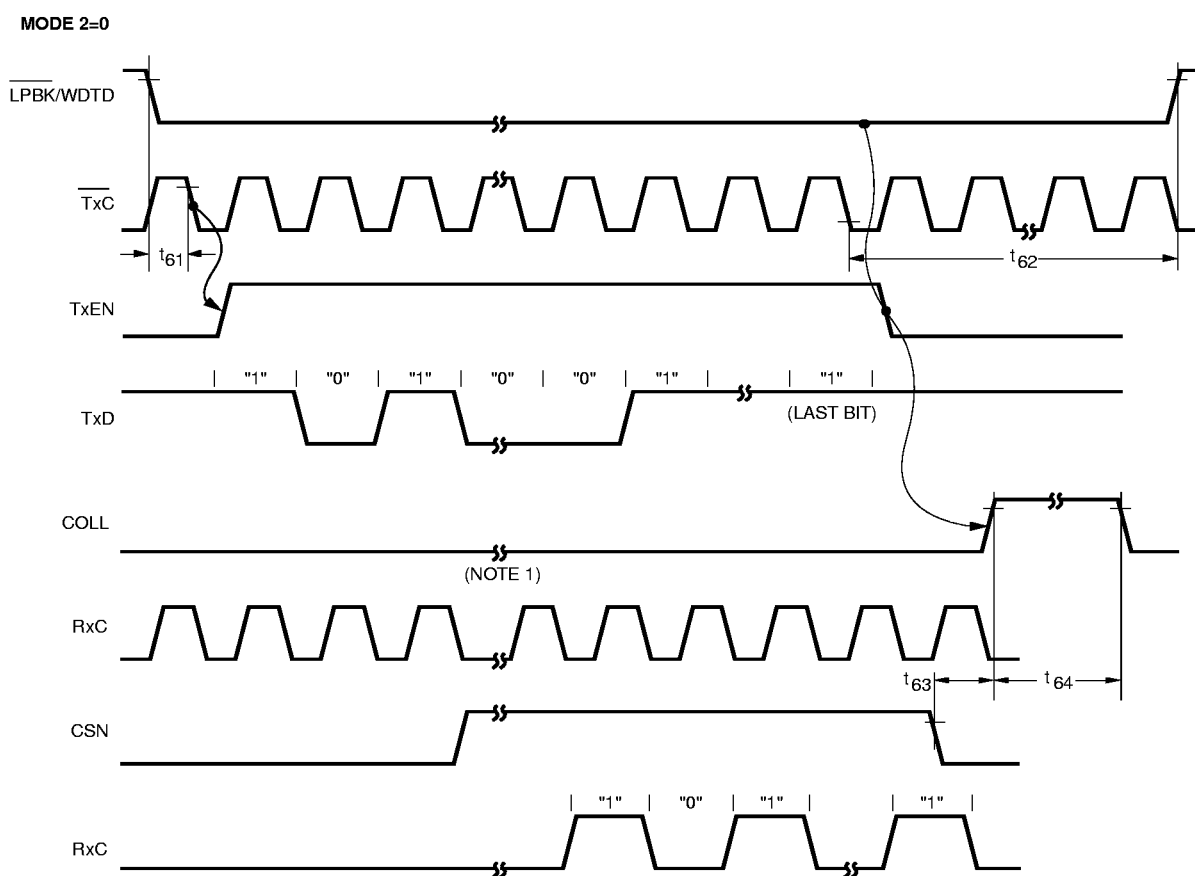
Figure 12. Loopback Timing
