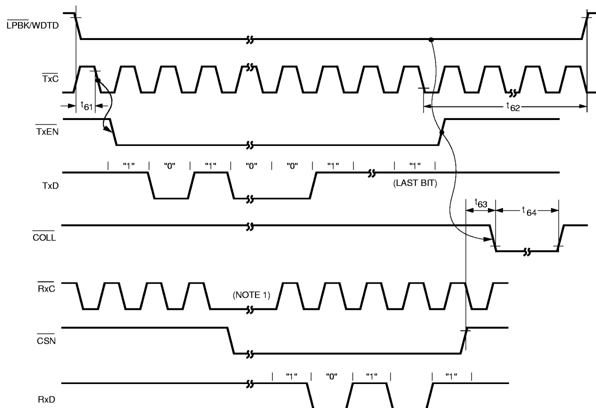
Figure 13. Loopback Timing —(Cont.)
