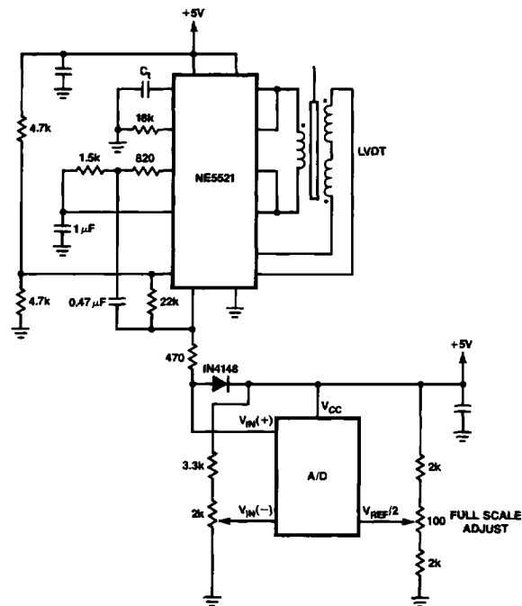
Figure 10. Digitizing a Transducer Interface Output
