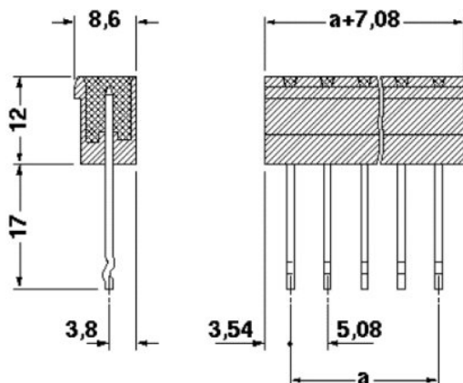
Dimensioned drawing
