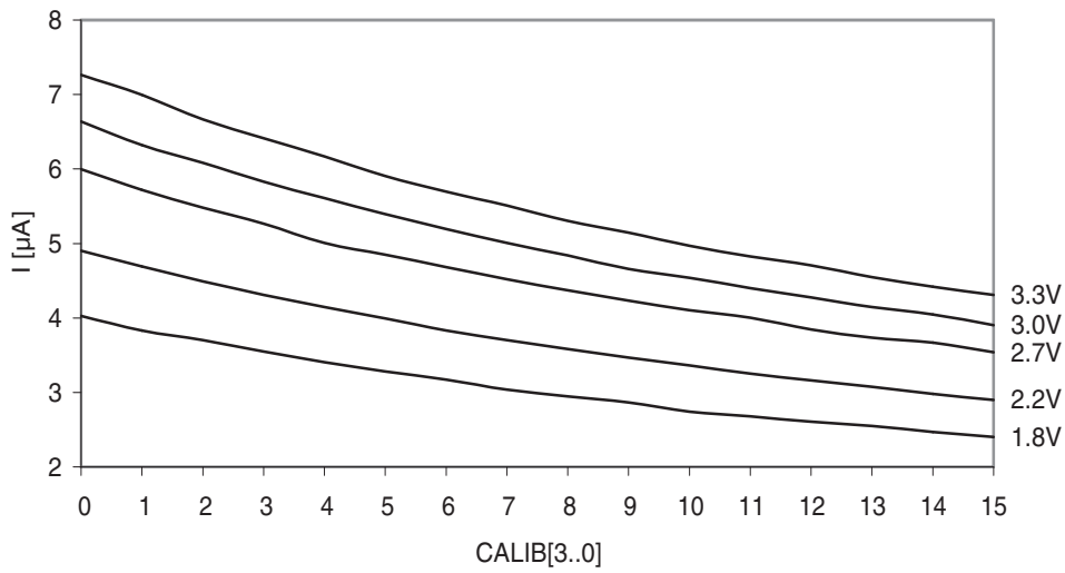
Figure 37-221. Analog comparator current source vs. calibration value.
