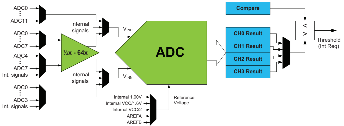
Figure 28-1. ADC overview.
