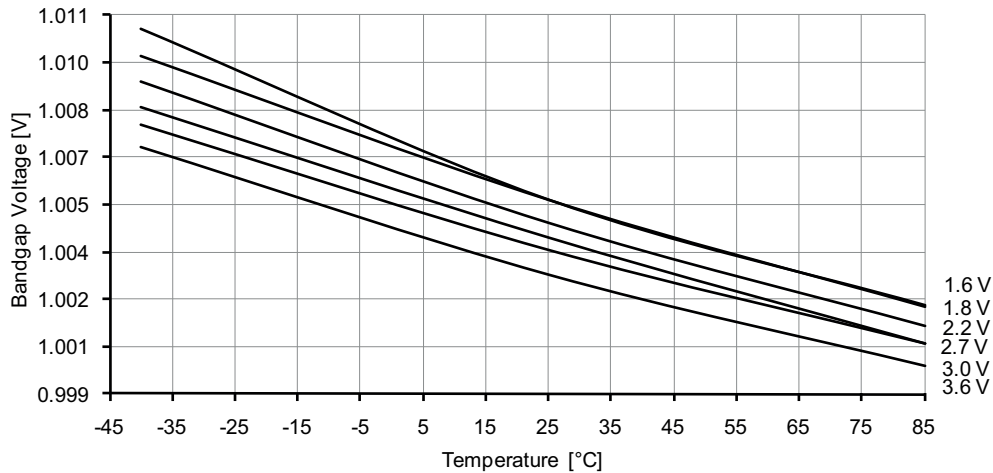
Figure 37-58. ADC/DAC Internal 1.0V reference vs. temperature.
