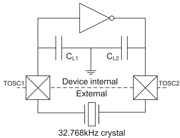
Figure 36-25.TOSC input capacitance.
