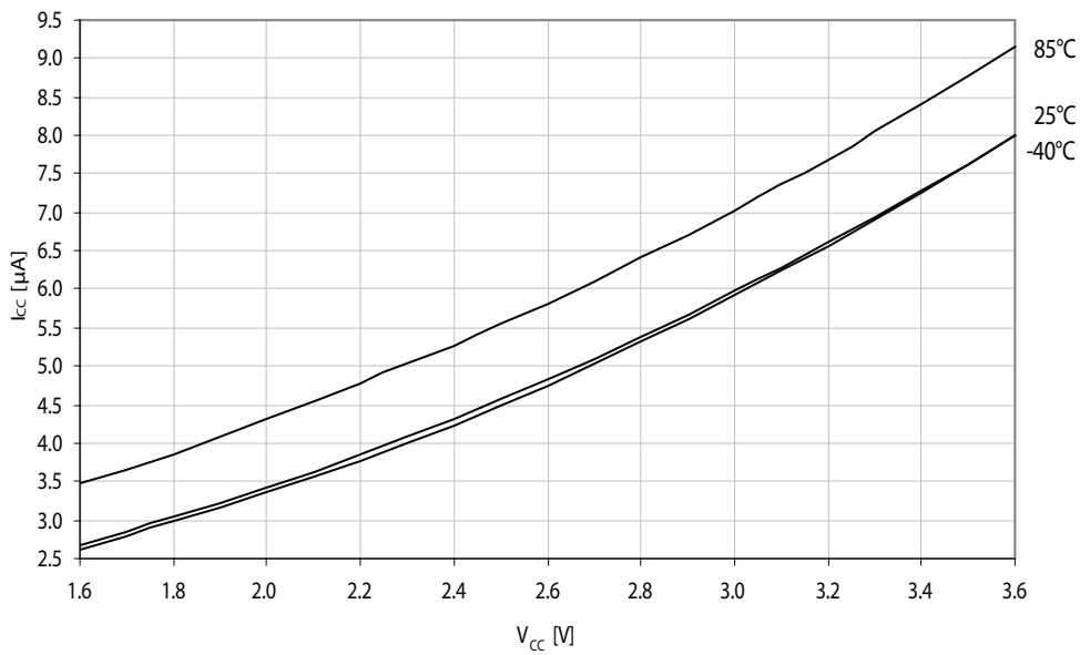
Figure 37-101. Standby supply current vs. V_{CC} . Standby, f_{SYS} = 1MHz .
