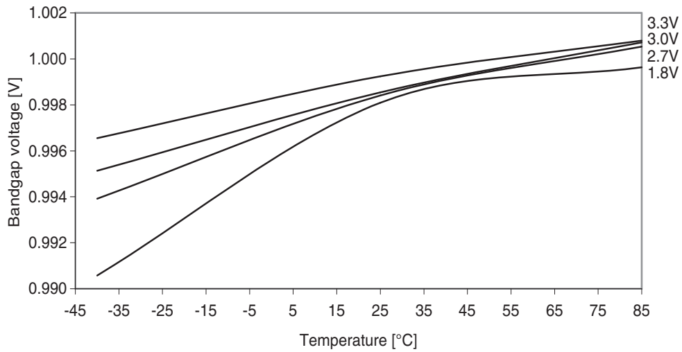
Figure 37-307. ADC/DAC Internal 1.0V reference vs. temperature.
