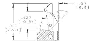
SHORT LATCH EJECTOR for IDS2 without strain relief
