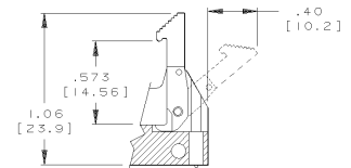
LONG LATCH EJECTOR for IDS2 with strain relief
