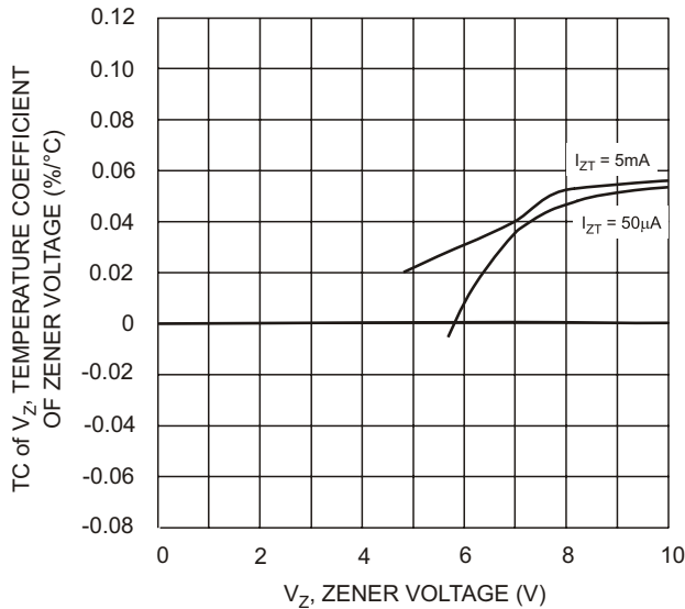
Fig. 16 Typical Temperature Coefficient of Zener Voltage vs. Zener Voltage, DDZX9690 - DDZX9697
