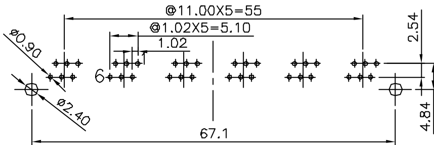
PC Board Layout Component Side Shown
