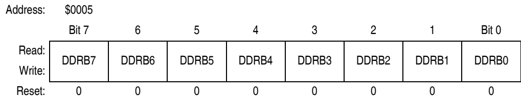
Figure 12-6. Data Direction Register B (DDRB)
