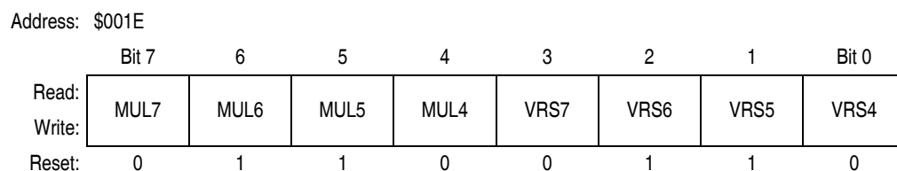
Figure 5-6. PLL Programming Register (PPG)
