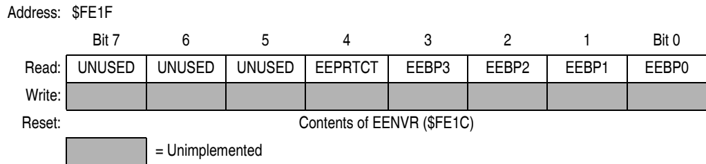
Figure 2-4. EEPROM Array Configuration Register (EEACR)
