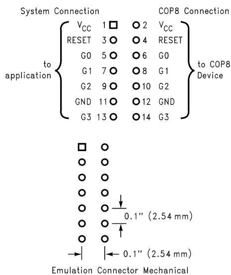
FIGURE 6. Emulation Connection
