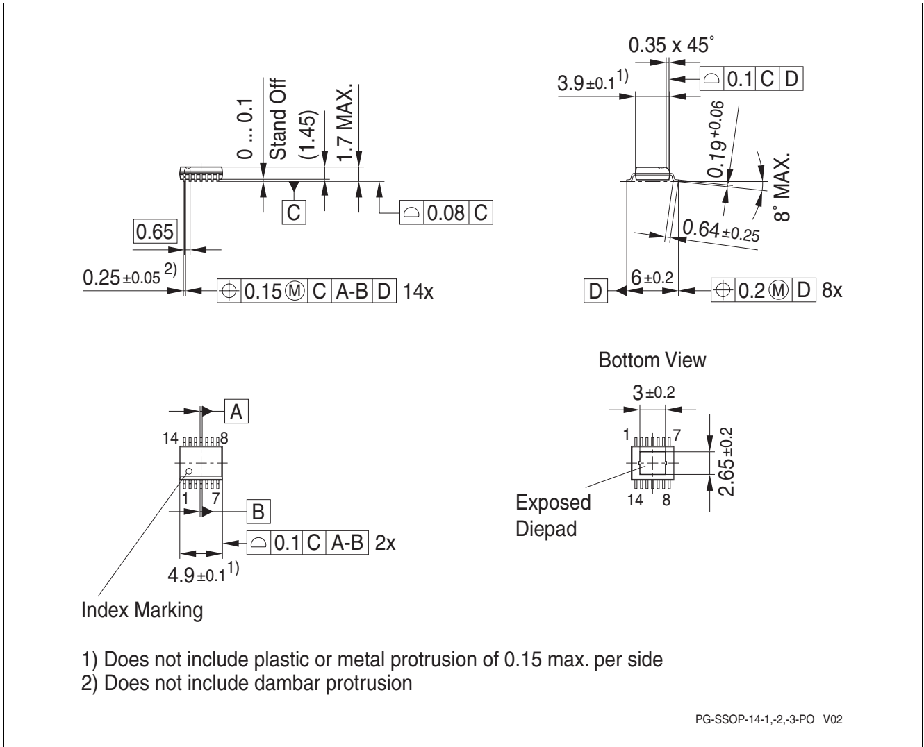
Figure 3 PG-SSOP-14 Exposed Pad
