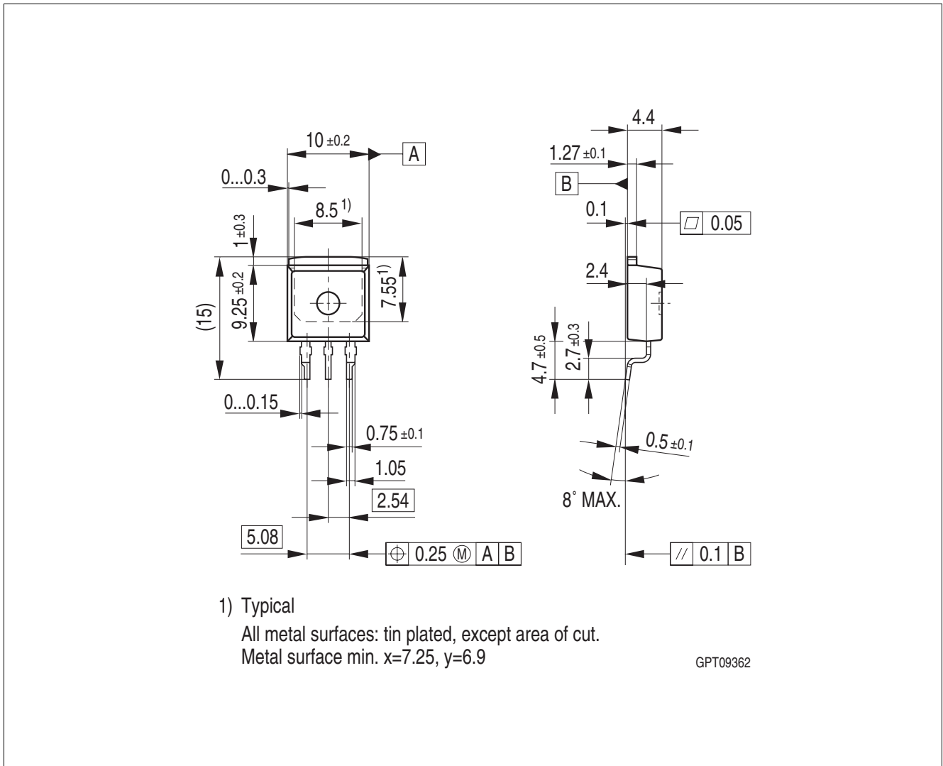
Figure 5 PG-TO263-3
