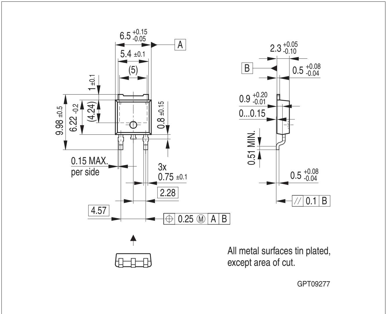
Figure 4 PG-TO252-3
