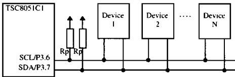
Figure 15. Typical I 2 C bus configuration
