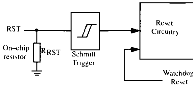
Figure 5. On-Chip Reset Configuration.
