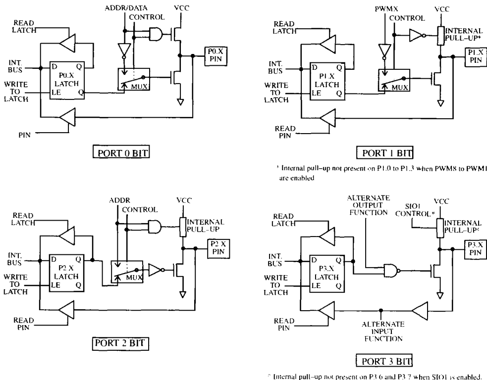
Figure 4. Port Bit Latches and I/O buffers
