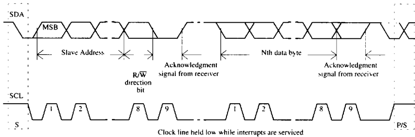
Figure 16. Complete data transfer on I 2 C bus
