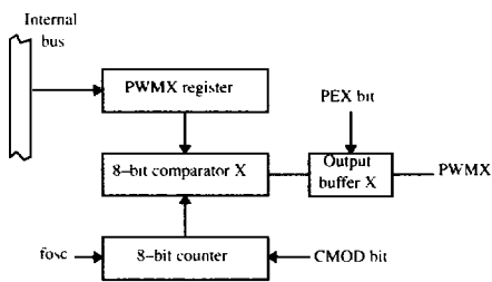
Figure 10. Pulse width modulated outputs block diagram
