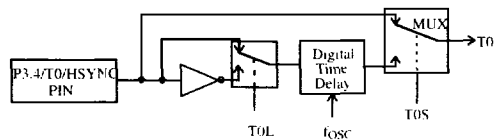
Figure 14. T0/HSYNC input block diagram
