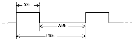
Figure 11. PWM programming example.
