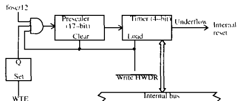
Figure 9. Watchdog timer block diagram
