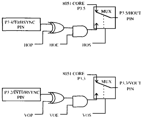
Figure 12. Buffered HSYNC and VSYNC block diagram
