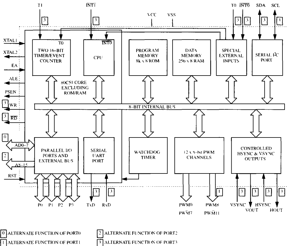
Figure 1. TSC8051C1 block diagram.
