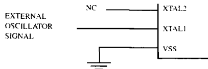
Figure 8. External Drive Configuration
