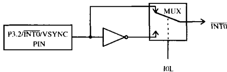
Figure 13. \overline{\text{INT0}}/\text{VSYNC} input block diagram
