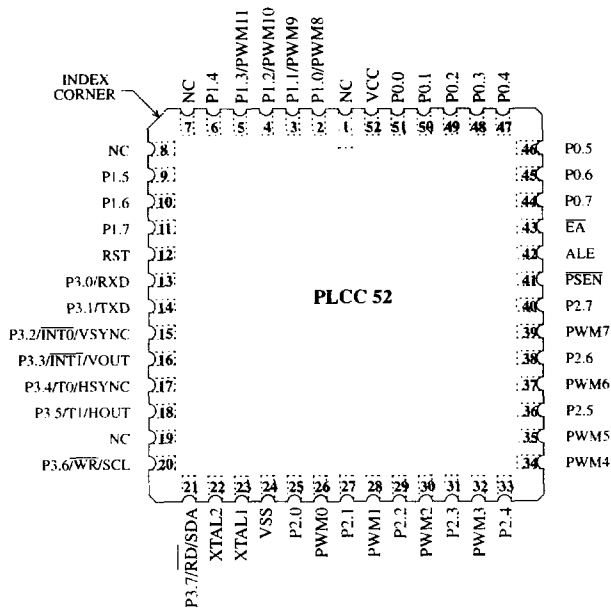
Figure 2. TSC8051C1 pin configurations.
