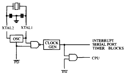
Figure 3. Idle and Power Down Hardware.
