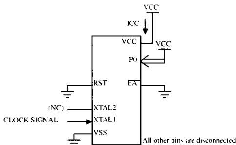
Figure 18. ICC Test Condition, Idle Mode.
