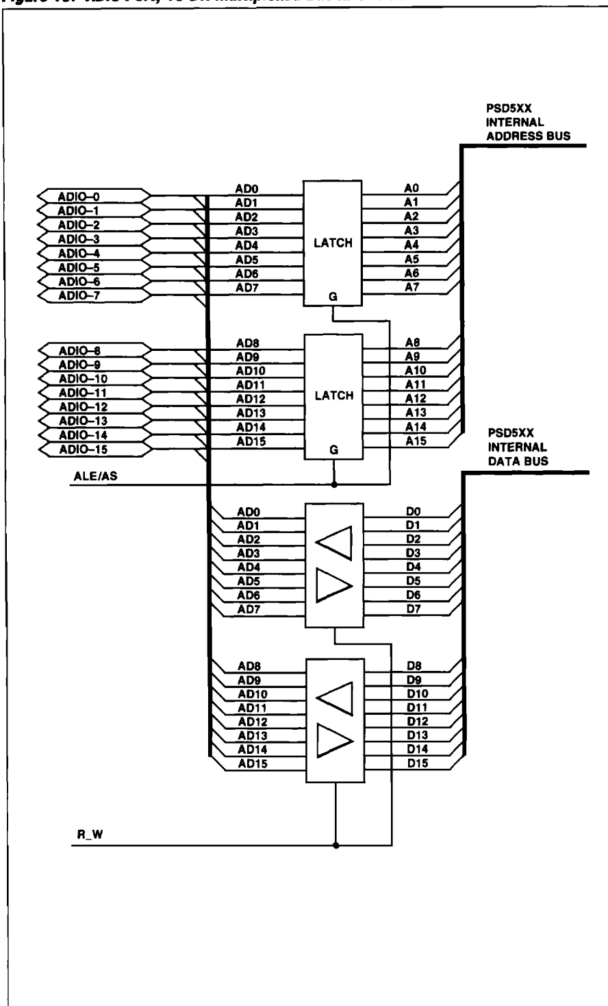
Figure 15. ADIO Port, 16-Bit Multiplexed Bus Interface
