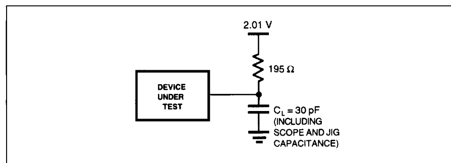
Figure 63. AC Testing Load Circuit
