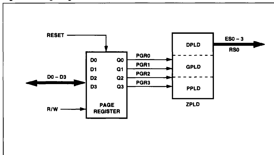
Figure 30. Page Register
