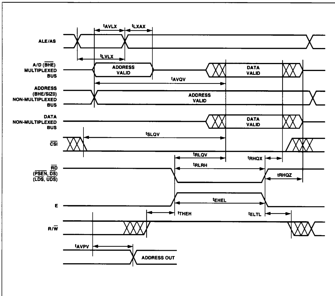
Figure 51. Read Timing
