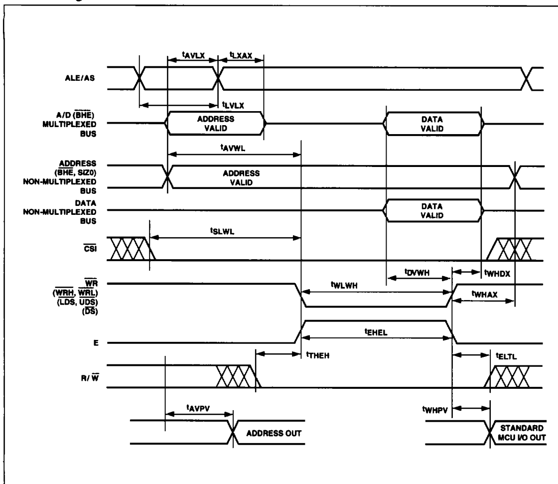
Figure 52. Write Timing
