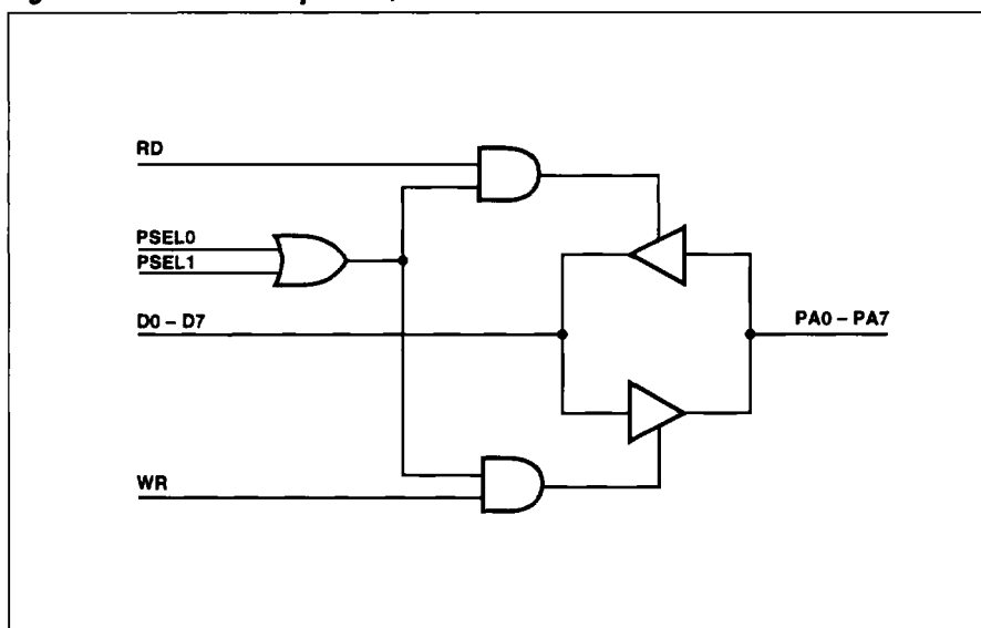
Figure 28. Port A In Peripheral I/O Mode
