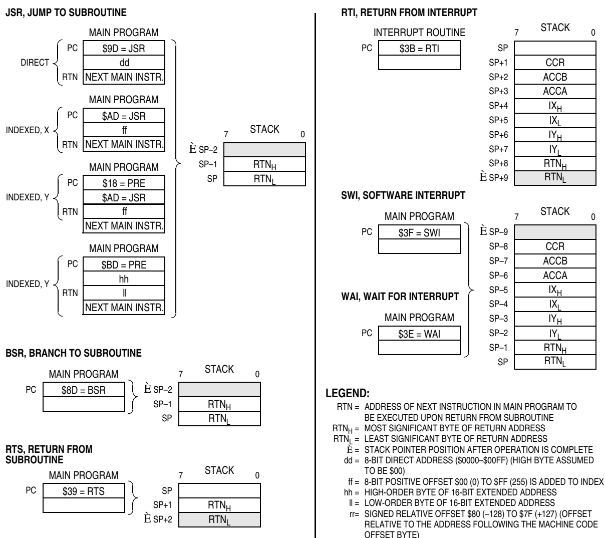
Figure 4-2. Stacking Operations
