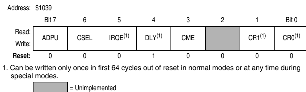
Figure 2-13. System Configuration Options Register (OPTION)
