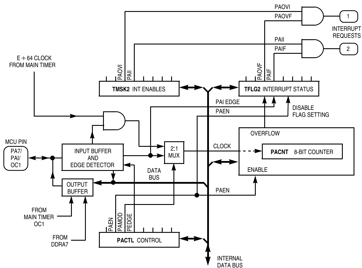
Figure 9-24. Pulse Accumulator
