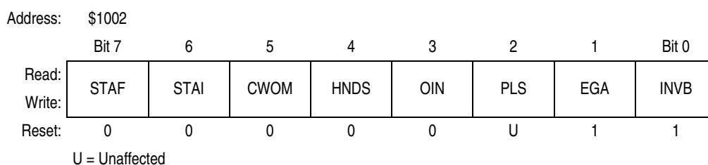
Figure 6-10. Parallel I/O Control Register (PIOC)
