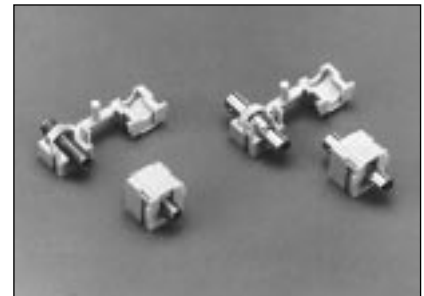
SMA/ST fiber optic couplers with adapters
