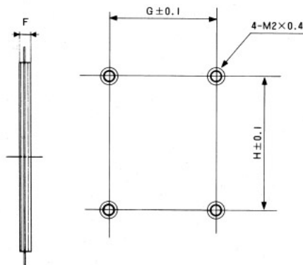
PCB Mounting Pattern
