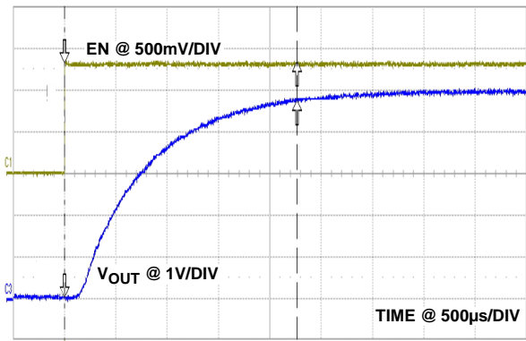
FIGURE 8. START-UP WAVEFORM
