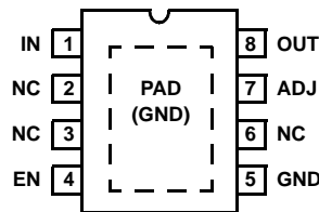
ISL80136 (8 LD EPSOIC) TOP VIEW
