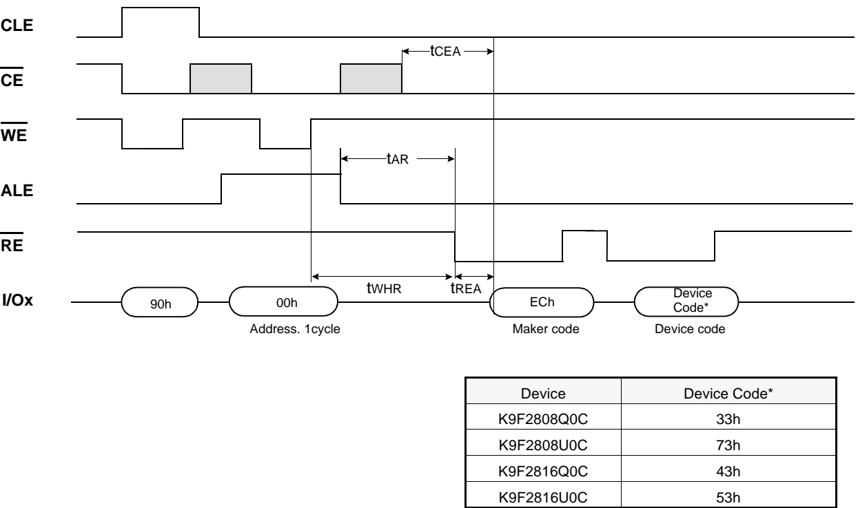
Figure 12. Read ID Operation
