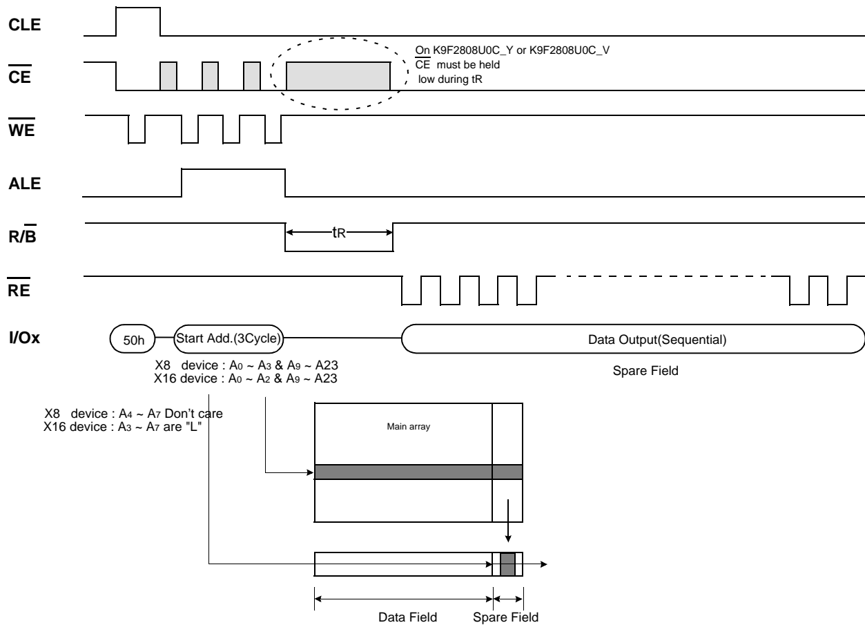
Figure 8-1. Sequential Row Read1 Operation (only for K9F2808U0C-Y and K9F2808U0C-V, valid within a block )
