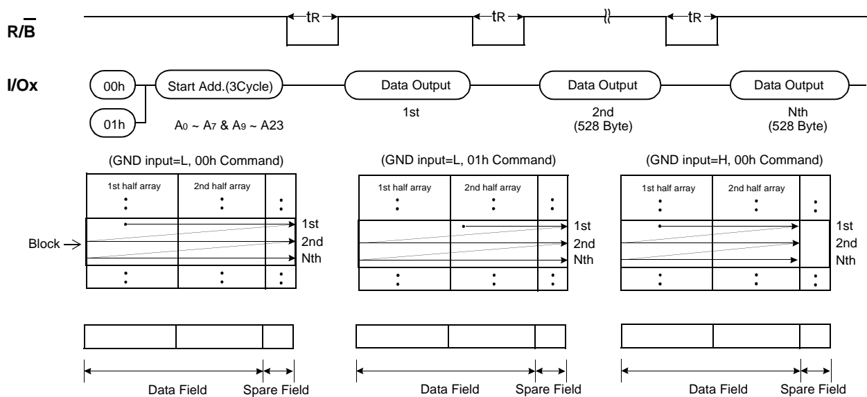
Figure 8-1. Sequential Row Read1 Operation (only for K9F2808U0C-Y and K9F2808U0C-V, valid within a block )
