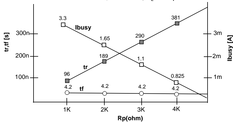
Fig 14 R_p vs t_r, t_f & R_p vs i_{busy}
