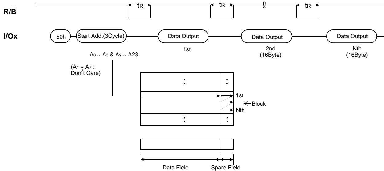
Figure 9-1. Sequential Row Read2 Operation (GND Input=Fixed Low) (only for K9F2808U0C-Y and K9F2808U0C-V, valid within a block)
