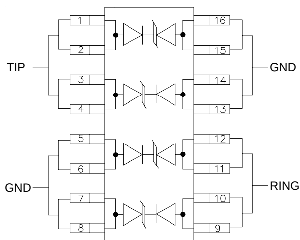
Figure 2 - Connection for Common Mode (Line-to-Ground) Protection of one Tip/Ring Line Pair
