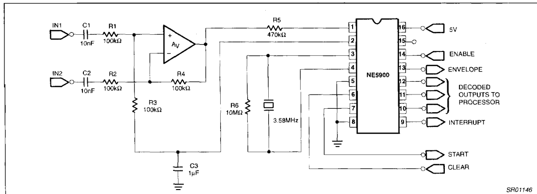
Figure 5. Typical Two-Wire Application
