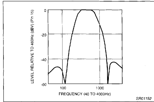
Figure 11. Filter Frequency Response
