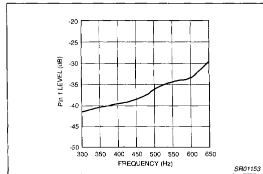
Figure 12. Typical Threshold
