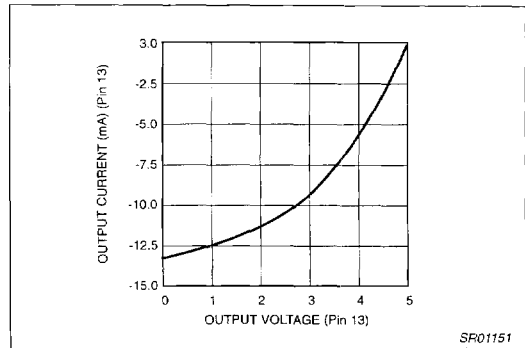
Figure 10. Output Voltage Current Curve Digital Output High
