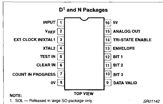
Figure 1. Pin Configuration
