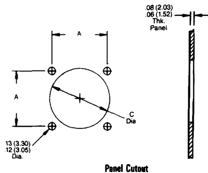
Panel Cutout
