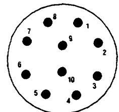
SLC-10 Face view, plug side
