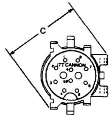
Front-Face View 10 Cavity Housing
