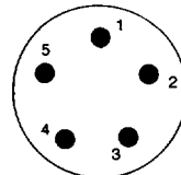
SLC-5 Face view, plug side
