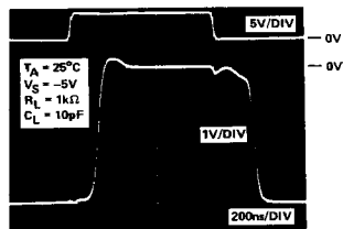
SW-201 t_{ON}/t_{OFF} SWITCHING RESPONSE
