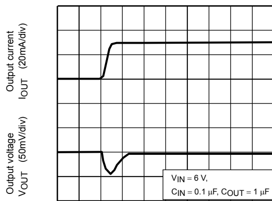
TCR5SB50U ( I_{OUT} = 1\text{m to }30\text{mA} )
