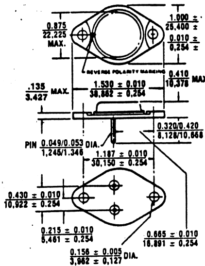
All dimensions in \frac{\text{INCH}}{\text{m.m.}} FIGURE 1
