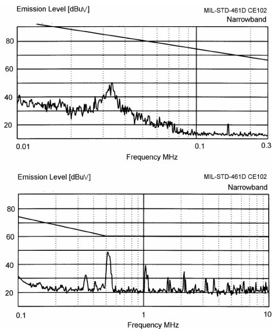
Figure 12 – MIL-STD-461D DVETR2800S
