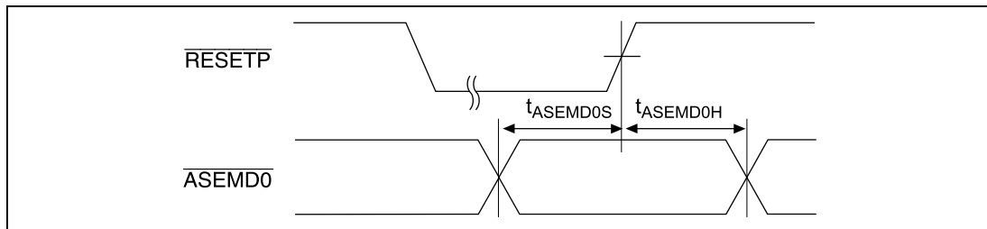
Figure 23.58 \overline{\text{ASEMD0}} Input Timing
