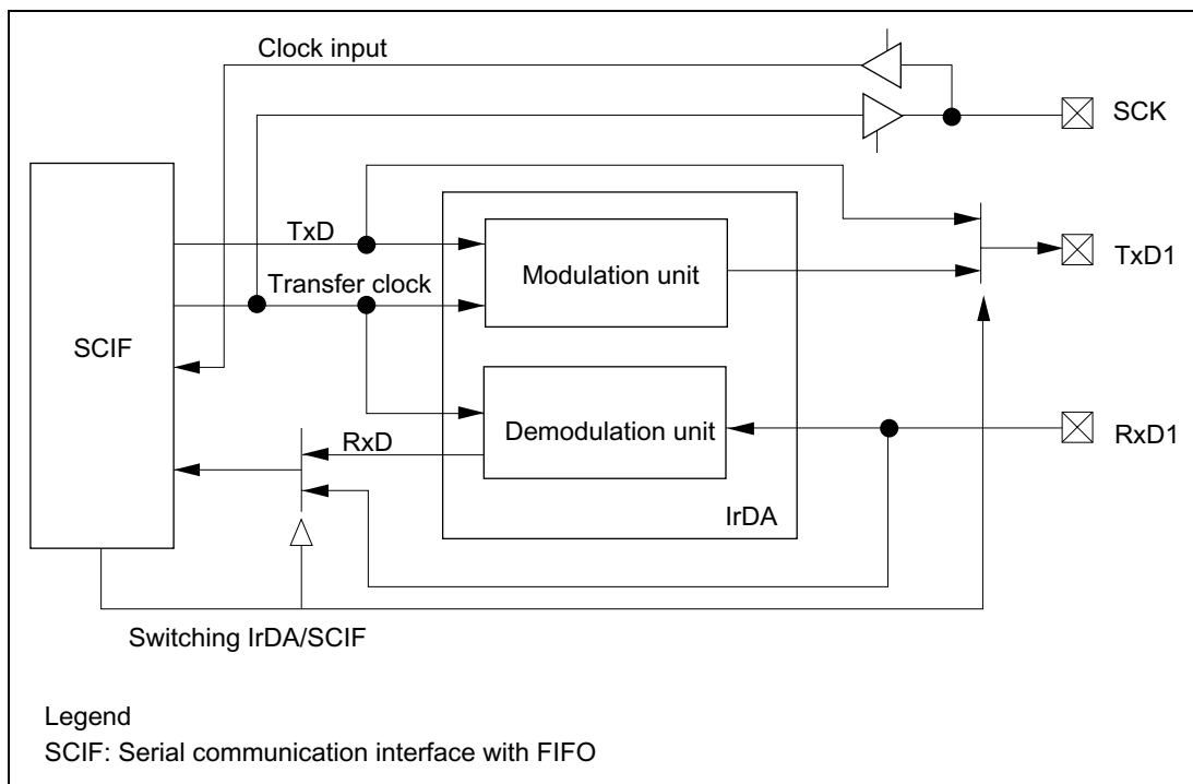
Figure 17.1 Block Diagram of IrDA
