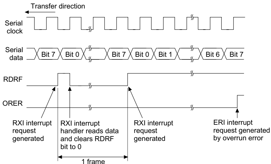
Figure 14.22 Example of SCI Receive Operation
