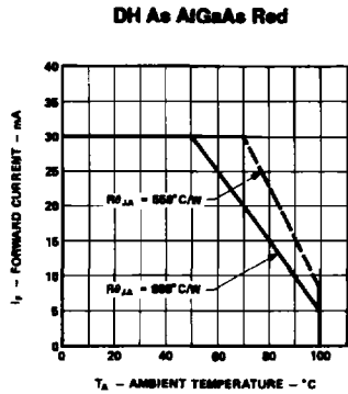
Figure 5. Maximum Forward dc Current vs. Ambient Temperature. Derating Based on T J MAX = 110 °C.
