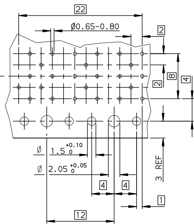
LAYOUT FOR P.C.B
