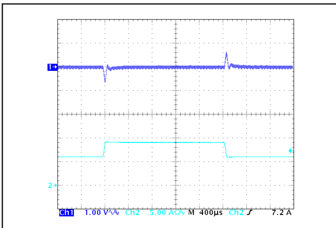
Figure 5: Output voltage response to step-change in load current (50%-75%-50% of Iout(max); dl/dt = 0.1 A/µs). Load cap: 1 µF ceramic and 15 µF tantalum capacitors. Ch 1: Vout (1 V/div), Ch 2: Iout (5 A/div).
