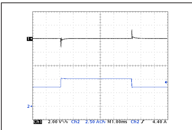
Figure 5: Output voltage response to step-change in load current (50%-75%-50% of I out (max)); dI/dt = 0.1 A/μs. Load cap: 1 μF ceramic and 15 μF tantalum capacitors. Ch 1: V out (2 V/div), Ch 2: I out (2.5 A/div).
