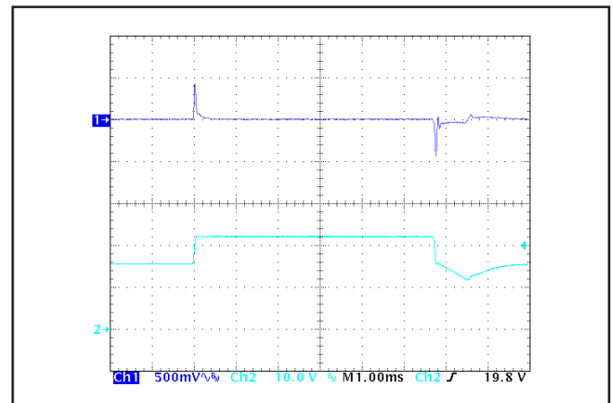
Figure 6: Output voltage response to step-change in input voltage (500 V/ms). Load cap: 100 µF, electrolytic output capacitance. Ch 1: Vout (500 mV/div), Ch 2: Vin (10 V/div).
