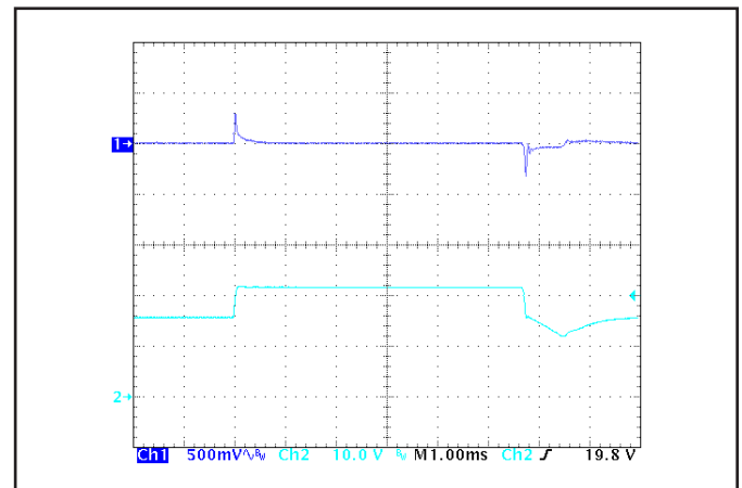
Figure 6: Output voltage response to step-change in input voltage (500 V/ms). Load cap: 100 \mu\text{F} , electrolytic output capacitance. Ch 1: Vout (500 mV/div), Ch 2: Vin (10 V/div).
