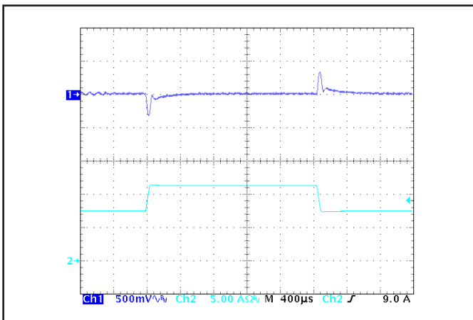
Figure 5: Output voltage response to step-change in load current (50%-75%-50% of Iout(max)); dl/dt = 0.1 \text{ A}/\mu\text{s} . Load cap: 1 \mu\text{F} ceramic and 15 \mu\text{F} tantalum capacitors. Ch 1: Vout (500 mV/div), Ch 2: Iout (5 A/div).
