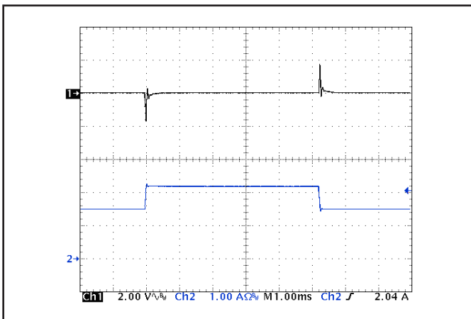
Figure 5: Output voltage response to step-change in load current (50%-75%-50% of I out (max); dl/dt = 0.05 A/μs). Load cap: 1 μF ceramic capacitor. Ch 1: V out (2 V/div), Ch 2: I out (1 A/div).
