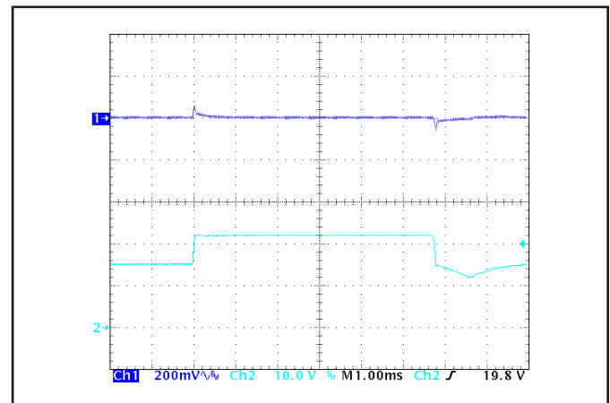
Figure 6: Output voltage response to step-change in input voltage (500 V/ms). Load cap: 100 \mu\text{F} , electrolytic output capacitance. Ch 1: V out (200 mV/div), Ch 2: V in (10 V/div).
