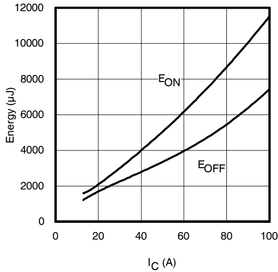
Fig. 13 - Typ. Energy Loss vs. I_C T_J = 150^\circ\text{C} ; L = 200\mu\text{H} ; V_{CE} = 600\text{V} ; R_G = 5.0\Omega ; V_{GE} = 15\text{V}
