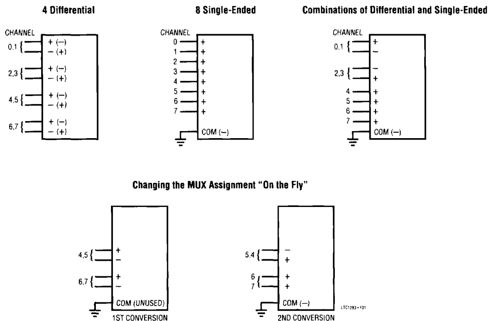
Figure 1. Examples of Multiplexer Options on the LTC1283
