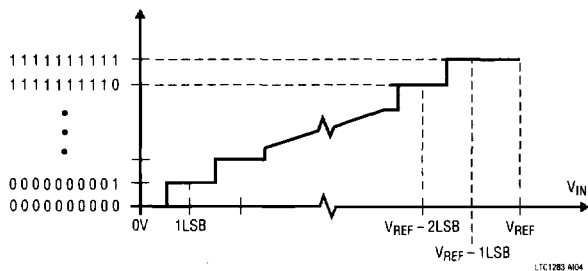
Unipolar Transfer Curve (UNI = 1)
