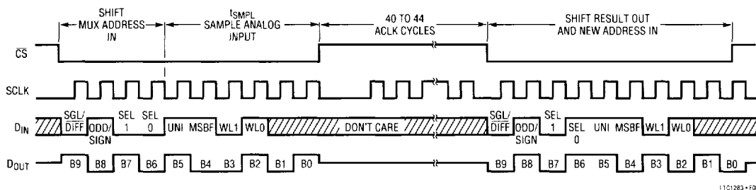
Figure 3. \overline{\text{CS}} High During Conversion
