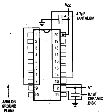
Figure 6. Example Ground Plane for the LTC1283
