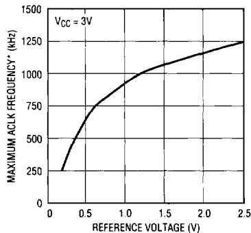
Maximum Conversion Clock Rate vs Reference Voltage
