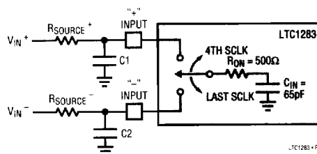
Figure 9. Analog Input Equivalent Circuit
