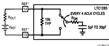
Figure 14. Reference Input Equivalent Circuit
