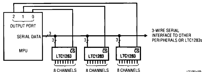
Figure 5. Several LTC1283s Sharing One 3-Wire Serial Interface
