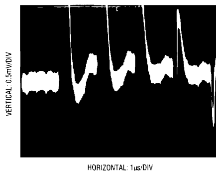
Figure 16. Poor Reference Settling Can Cause A/D Errors
