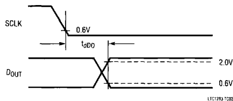
Voltage Waveforms for D_{OUT} Delay Time, t_{dDO}
