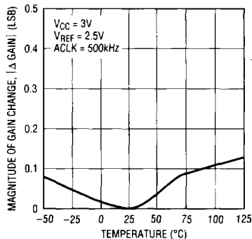
Change in Gain Error vs Temperature
