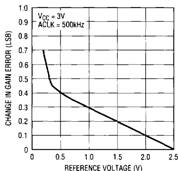
Change in Full-Scale Error vs Reference Voltage
