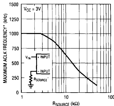
Maximum Conversion Clock Rate vs Source Resistance
