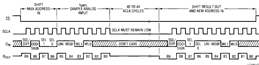
Figure 4. \overline{\text{CS}} Low During Conversion
