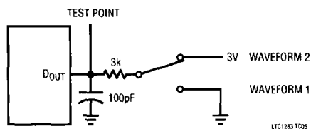
Load Circuit for t_{dis}
