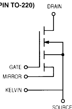
CASE 314B-02 (5 PIN TO-220)
