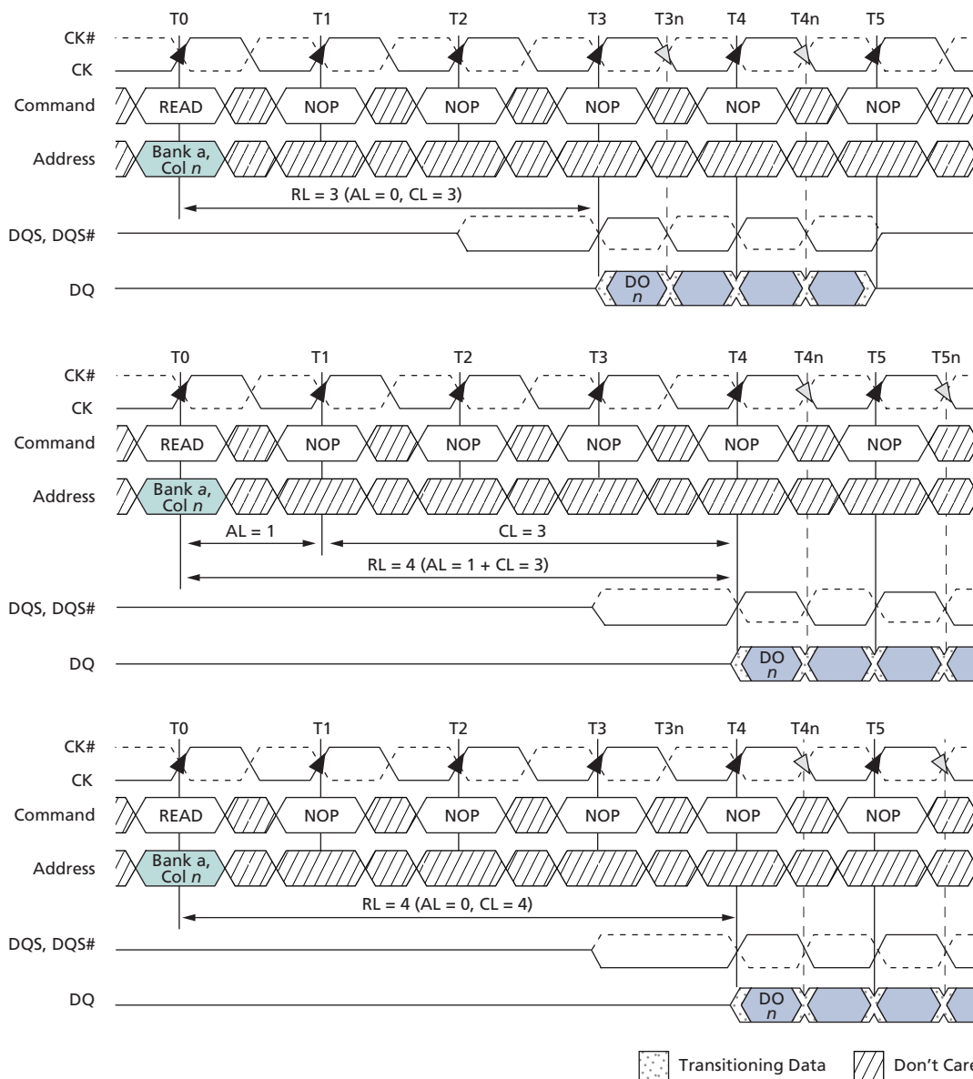
Figure 48: READ Latency
