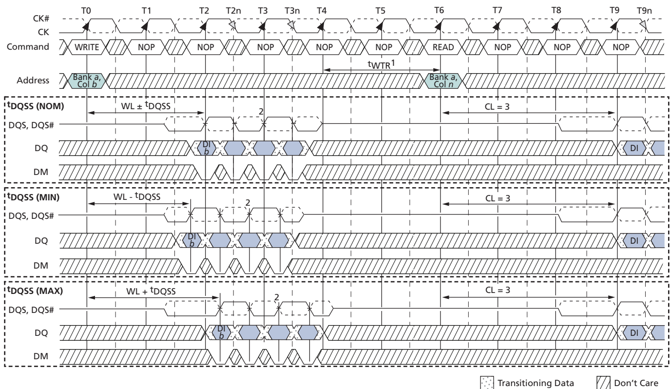
Figure 64: WRITE-to-READ
