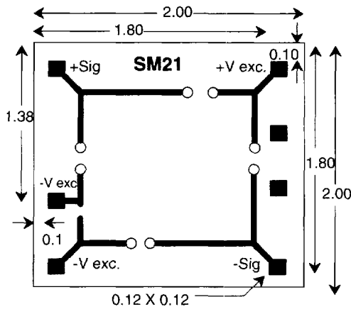
Figure 1. Layout
