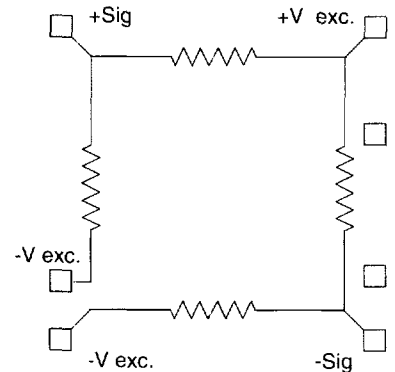
Figure 3. Schematic
